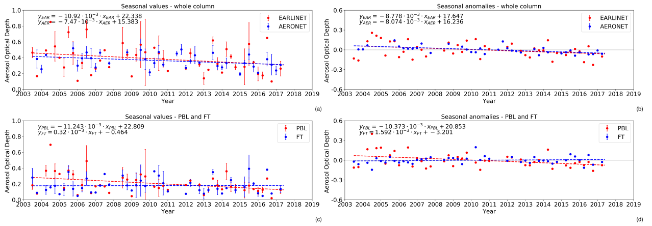
Timeseries of the AOD at 355nm over Thessaloniki
