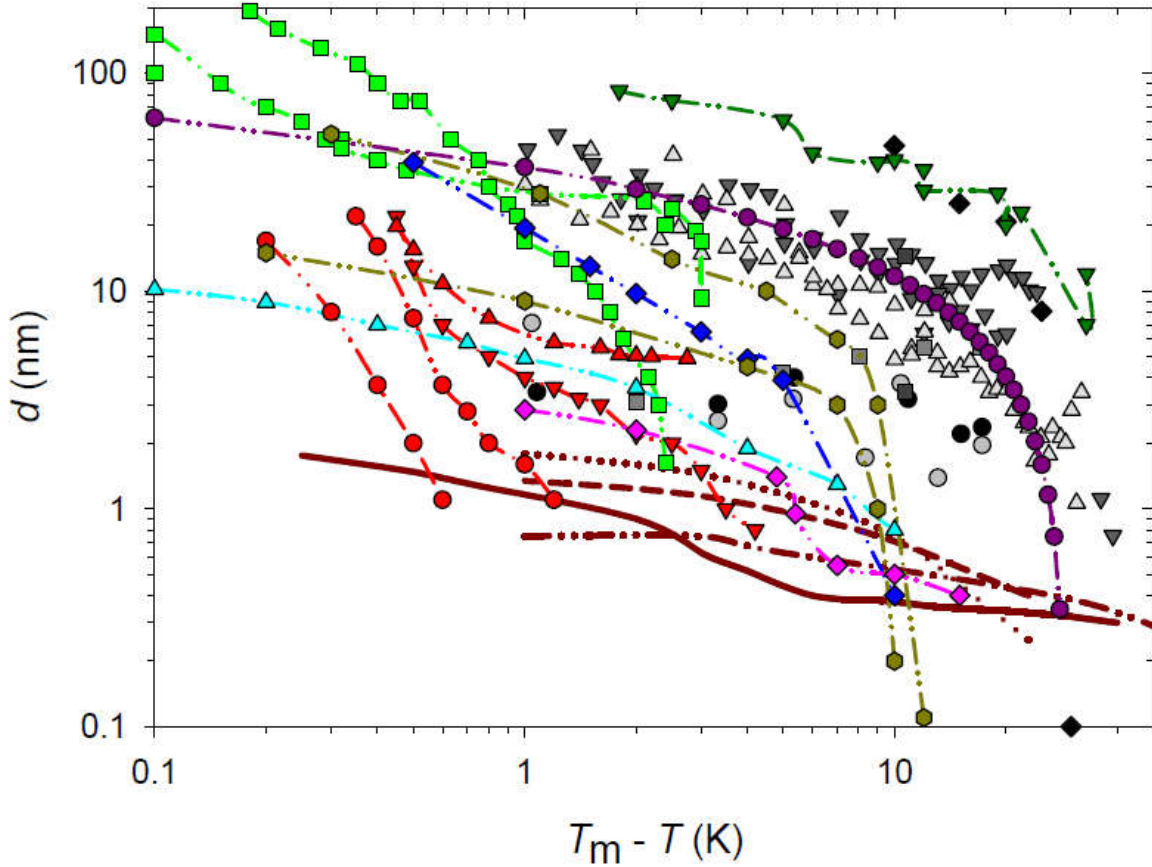
Figure 1: QLL thickness determined with different experimental and simulation techniques: AFM measurements by Pittenger et al. (Pittenger et al., 2001) with Si tips ( \bullet ) and hydrophobic coated silicon tips ( \bullet ); by Döppenschmidt et al. (Döppenschmidt et al., 2000) in air ( \blacktriangledown ) and vacuum ( \blacktriangle ); by Petrenko (Petrenko, 1997) ( \blacksquare ); by Bluhm et al. (BluhmandSalmeron, 1999 and Bluhm et al., 2000) ( \blacksquare ). IFM measurements by Goertz et al. (Goertz et al., 2009) ( \blacklozenge ). Brewster reflectometry by Elbaum et al. (Elbaum et al., 1993) ( \bullet , \blacktriangle , \blacktriangledown ; different symbols correspond to different experiments). Ellipsometry by Beaglehole and Nason (Beaglehole and Nason, 1980) ( \blacklozenge ), and Furukawa et al. (Furukawa et al., 1987) ( \blacksquare ). XPS by Bluhm et al. (Bluhm et al., 2002) ( \blacklozenge ). FTIR by Sadtchenko and Ewing (Sadtchenko and Ewing, 2002) ( \blacktriangle ). Proton dispersion by Golecki and Jaccard (Golecki and Jaccard, 1977) ( \blacktriangledown ). GXR by Dosch et al. (Dosch et al., 1995 and 1996), and Lied et al. (Lied et al., 1994) ( \bullet , \bullet ). Simulation results by Limmer and Chandler (Limmer and Chandler, 2002) (—); Furukawa and Nada (Furukawa and Nada, 1997) (..... and - - -) for the prismatic and basal planes, respectively, and by Conde et al. (Conde et al., 2008) (- . - .) for the basal plane.
