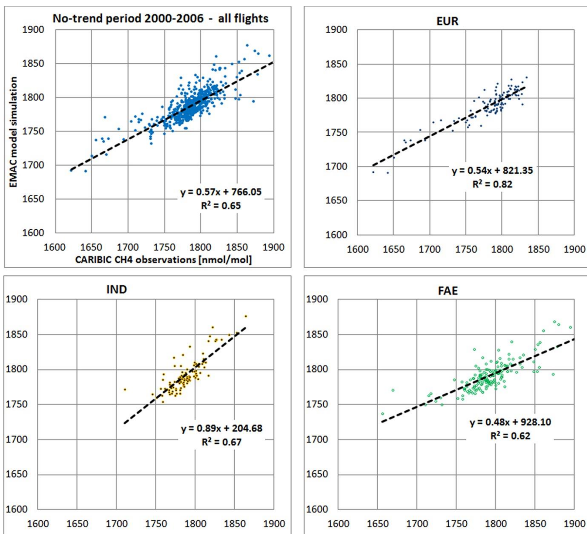
775 Figure 8: Correlation CARIBIC flight samples (x-axis) vs. EMAC simulations (y-axis) [nmol/mol] for all flights during no-trend period 2000 – 2006 (upper left) and the main flight regions India (IND), Europe (EUR), and Far East (FAE).
