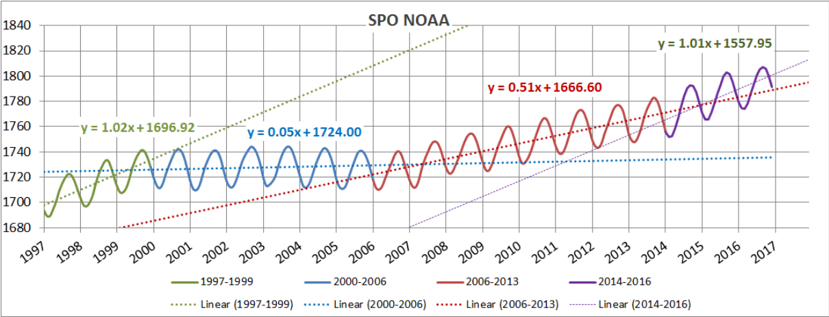
Figure 1: Development of monthly mean CH 4 mixing- ratios [nmol/mol] at the NOAA observation site South Pole (SPO, 90° S) over the years 1997 through 2016, the period considered in this modeling study.
