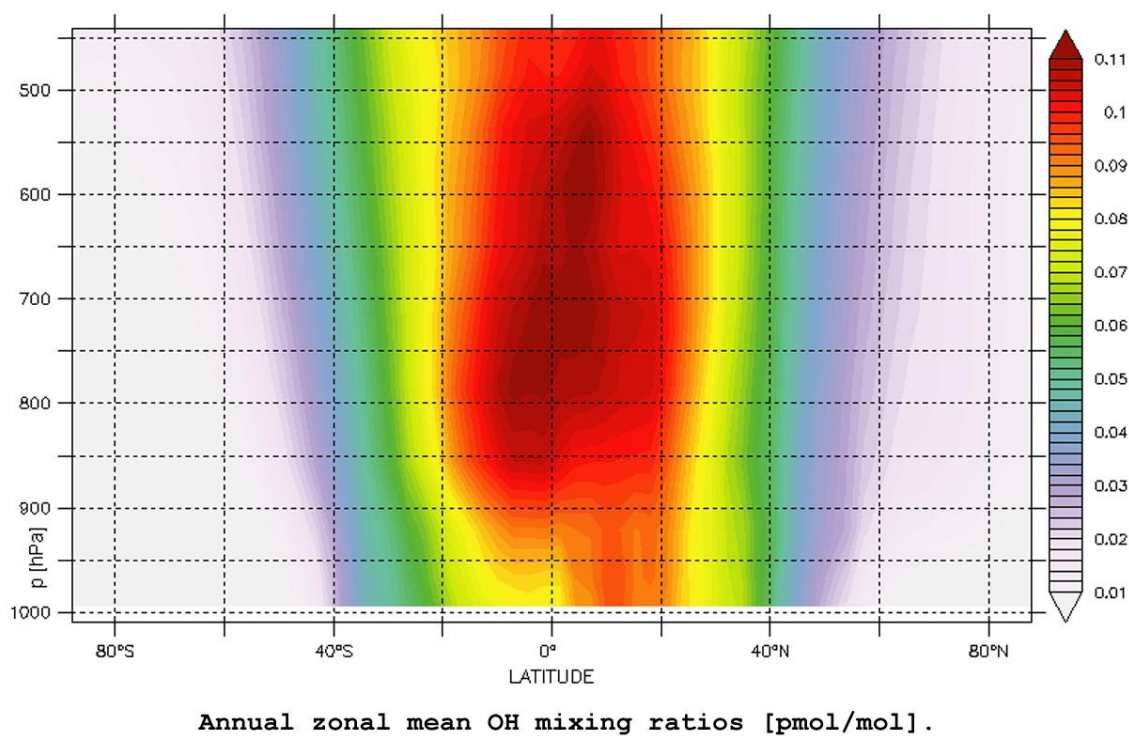
765 Figure 6: In the Northern Hemisphere lower troposphere the OH mixing-ratios are considerably higher than on the Southern Hemisphere
