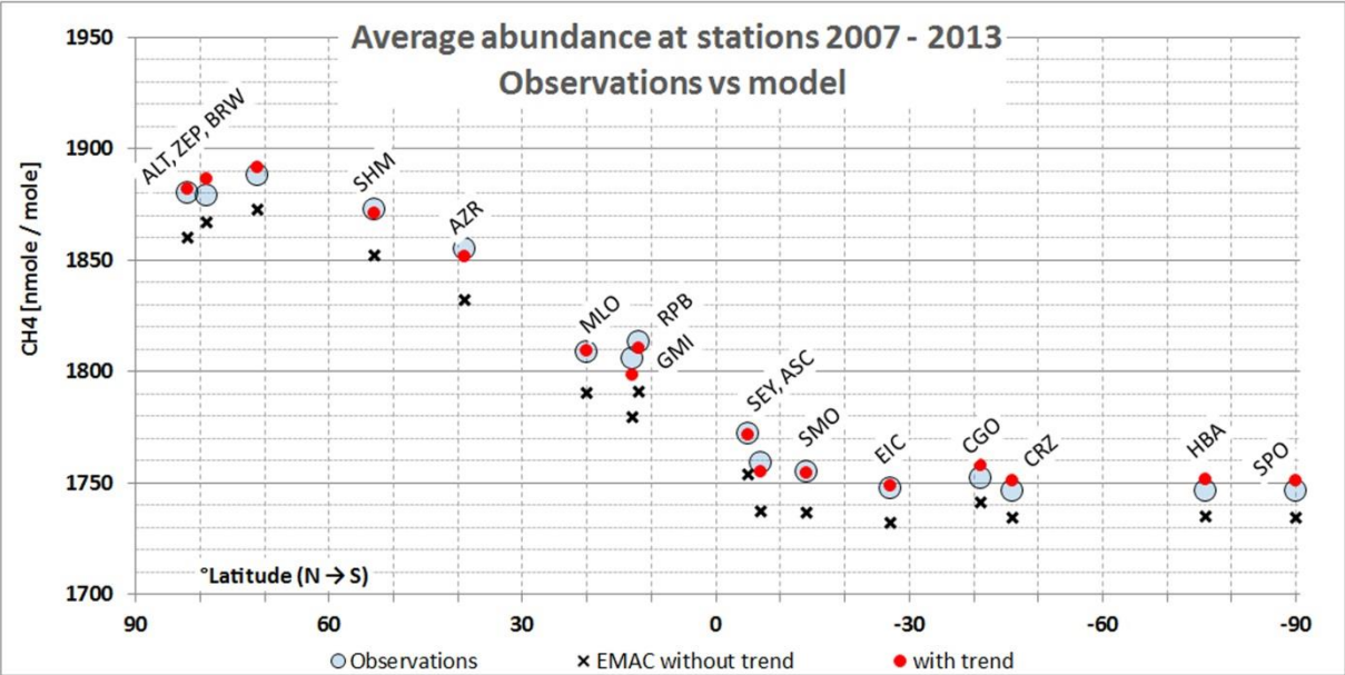
Figure 10: Calculated total CH 4 without- (black crosses), and with optimized trend period emissions (red dots). By scaling RIC, SHA, and TRO emission fractions, the station observations (blue circles) are approximated with smallest RMS. After 2013, the trend accelerates and additional emission assumptions are necessary.
