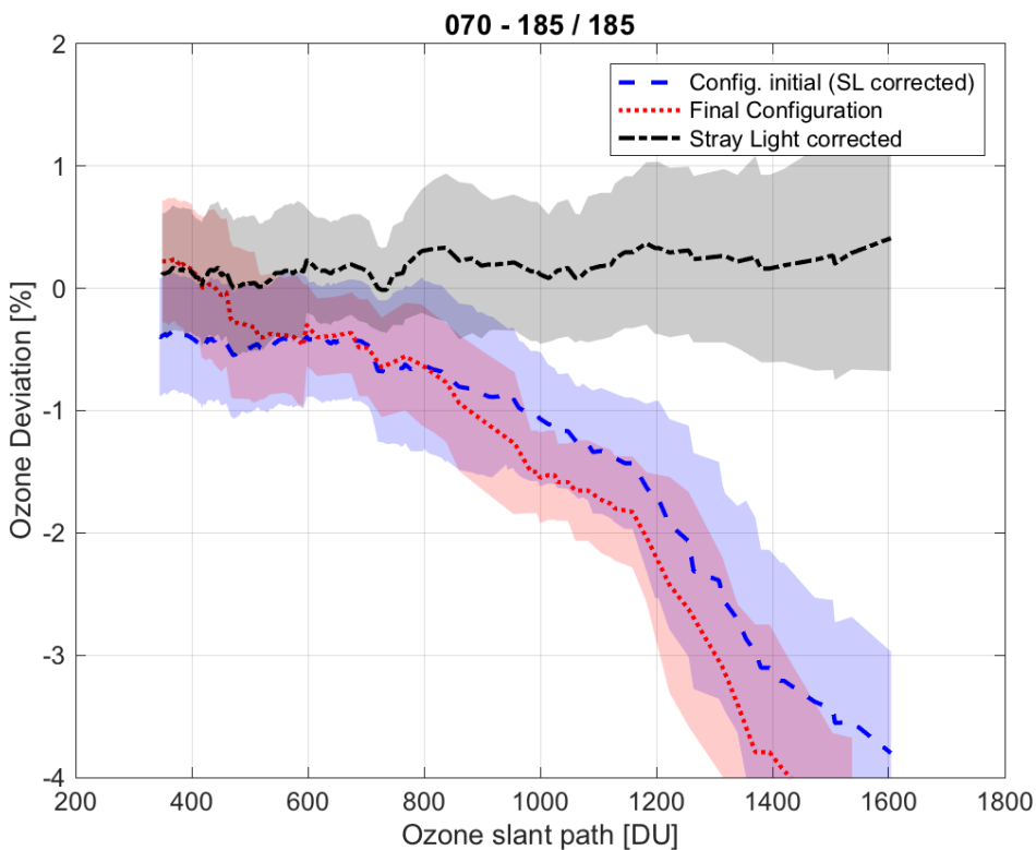
10 Figure 1: A comparison of a single Brewer, #070, with the RBCC-E reference Brewer, #185, showing stray light correction. The blue and red lines are the initial ozone deviation of #070 from the reference before and after calibration. The black line shows the stray light corrected values.
