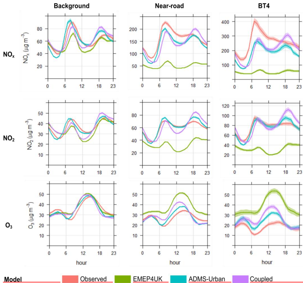
Figure 1342: Diurnal temporal variations of NO x , NO 2 and O 3 concentrations for the average over all background and near-road sites, and for an individual near-road site, with observations and modelled concentrations from each model. Note different concentration axis limits for each plot. The shaded area around the central line shows the 95% confidence interval in the mean.
