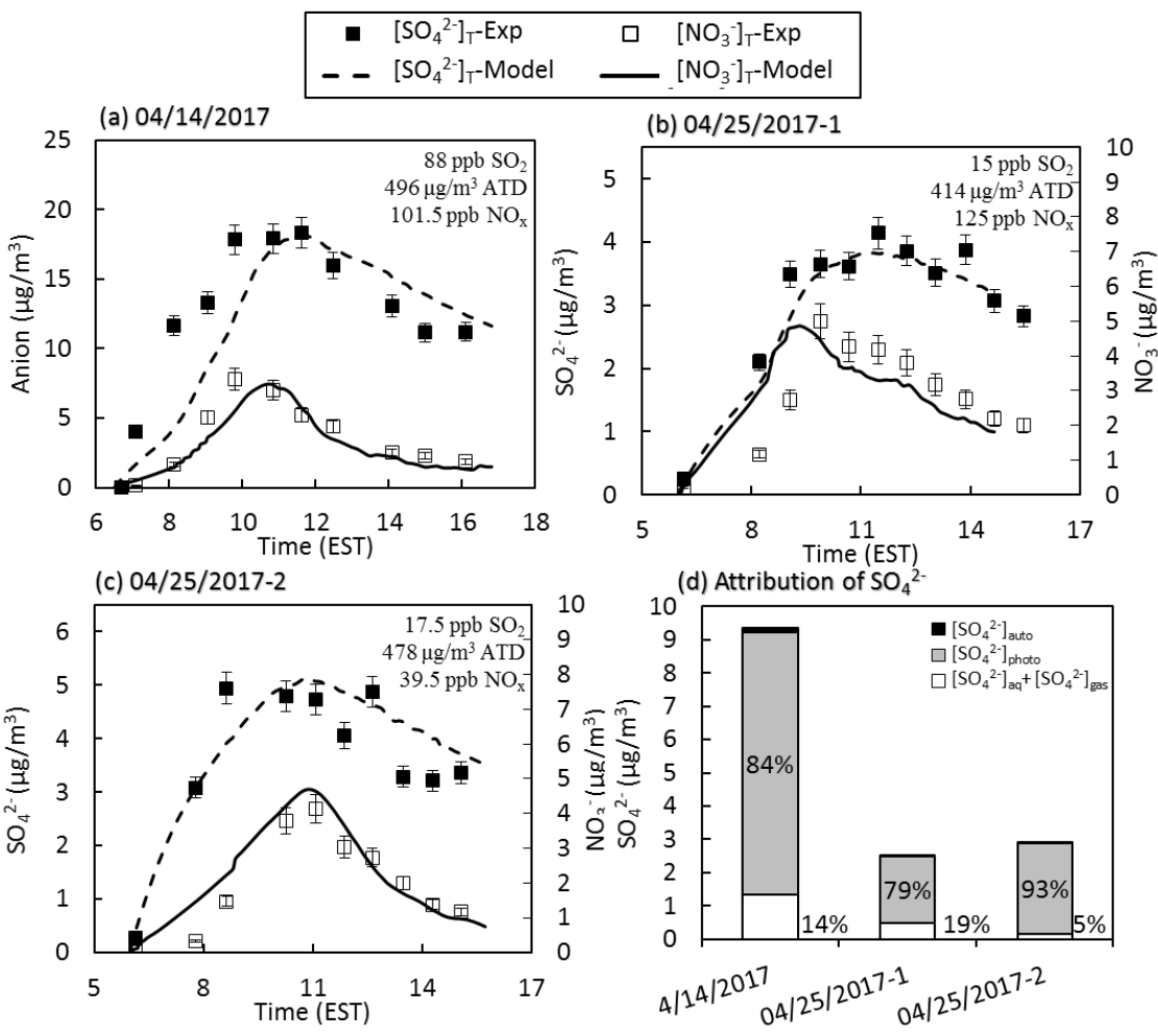
Figure 4. Time profiles of total sulfate concentration ( [\text{SO}_4^{2-}]_T , \mu\text{g}/\text{m}^3 ) and nitrate concentration ( [\text{NO}_3^-]_T , \mu\text{g}/\text{m}^3 ) in the dual chamber experiments using UF–APHOR at different \text{NO}_x levels.
