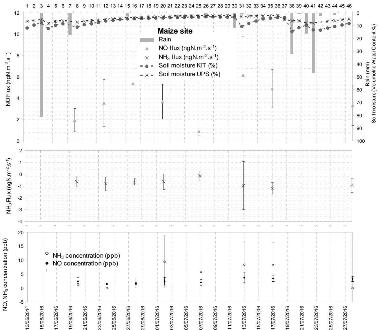
910 Fig. 4 Upper panel: Daily total precipitation (mm), daily mean soil moisture at 5 cm (%) measured by the Karlsruhe Institute of Technology (KIT), daily mean soil moisture averaged between 0 and 30 cm measured by the Université Paul Sabatier (UPS) instrumentation, daily mean NO fluxes in \text{ngN m}^{-2} \text{s}^{-1} measured at the maize field site ; Middle panel: daily mean NH 3 fluxes in \text{ngN m}^{-2} \text{s}^{-1} ; Lower panel: daily mean NO and NH 3 concentrations in ppb. Vertical bars show the standard deviation from individual fluxes and concentrations.
