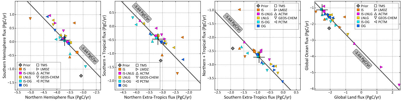
Figure 8. The partitioning of the 2015 global CO 2 sink into two geographical domains, with the tropics being defined as 23.5° north and south latitudes. This is similar to figure 7, except that we have compared two real OCO-2 and one real in situ sampling schemes (LNLG, OG, IS) with the two theoretical in situ ones (IS-LNLG, IS-OG) of § 2.3.3. The scales are identical across three of the four figures and the same as figure 7; the partitioning of global and ocean fluxes had significantly more spread, and required a different scale.
