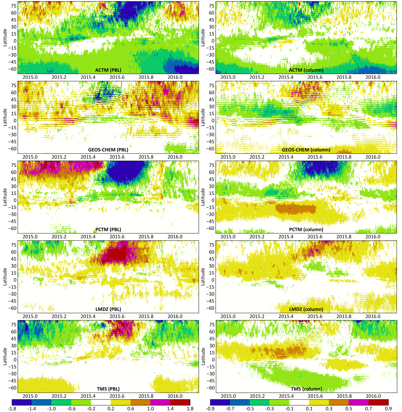
Figure 3. The zonal average difference between each model (ACTM, GEOS Chem, LMDZ, PCTM and TM5) and the cross-model median at 1:30 PM local time, in ppm \text{CO}_2 , between Dec 1 2014 (2014.915) and Mar 1 2016 (2016.164). The left column depicts differences in the lowest 150 hPa, which is an approximation for the PBL. The right column depicts differences in column averaged \text{CO}_2 . Each column has its own color bar. Since transport differences in the total column are smaller than in the PBL, the dynamic range of the right column is half that of the left column.
