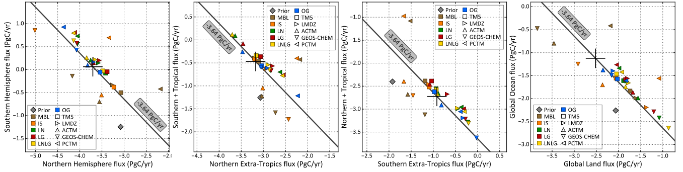
Figure 7. The partitioning of the 2015 global CO 2 sink into two geographical domains, with the tropics being defined as 23.5° north and south latitudes. Each color represents one type of synthetic data assimilated, while each symbol shape represents one model used to generate the synthetic data. The diagonal gray line represents the 2015 global sink of 3.64 PgC/yr in the true fluxes used to generate the synthetic data, while the large plus sign denotes their partitioning. The scales are identical across all four figures, but not the origins.
