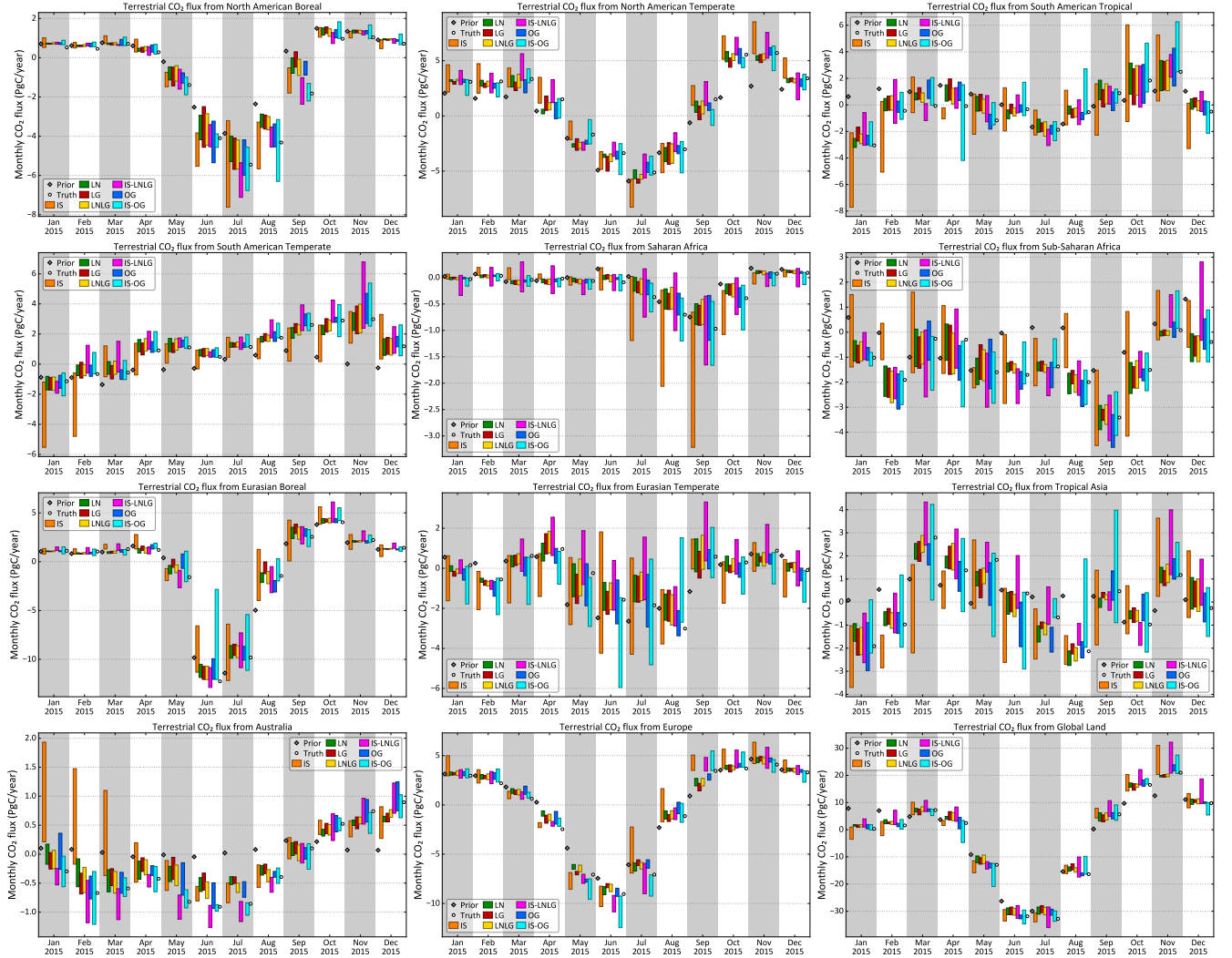
Figure 5. Monthly flux estimates from TRANSCOM-like land regions and global total land. The different colors correspond to different synthetic data streams assimilated, as in figure 4. The different models used to generate the synthetic data have not been distinguished here to minimise visual clutter. The theoretical PBL networks IS-LNLG and IS-OG have also been omitted for the same reason. Plots of seasonal fluxes over many more regions, with the models distinguished, are included in the supplementary material.
