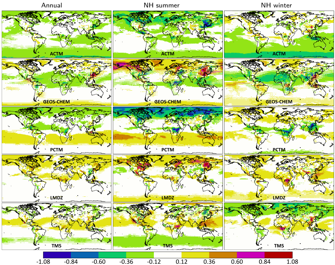
Figure B2. Same as figure B1, except averaged over the total column. The dynamic range here is half that of figure B1, since transport differences in the total column signal are smaller than in the PBL signal.
