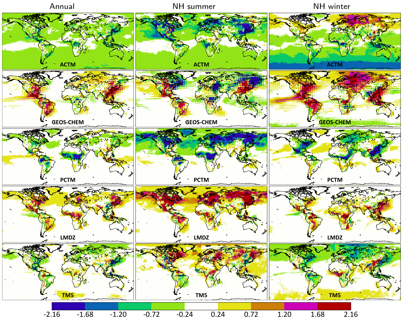
Figure B1. The difference between each model (ACTM, LMDZ, GEOS Chem, PCTM and TM5) and the cross-model median at 1:30 PM local time in the lowest 150 hPa, which is an approximation for the planetary boundary layer (PBL). The left column shows the difference averaged over all of 2015, the middle column is averaged over northern hemisphere summer months (Jun–Aug 2015), and the right column is averaged over northern hemisphere winter months (Dec 2015 to Feb 2016). Differences are shown in ppm CO 2 .
