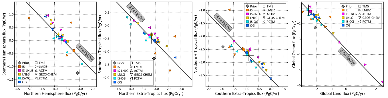
Figure 8. The partitioning of the 2015 global CO 2 sink into two geographical domains, with the tropics being defined as 23.5° north and south latitudes. This is similar to figure 7, except that we have compared two real OCO-2 and one real in situ sampling schemes (LNLG, OG, IS) with the two theoretical in situ ones (IS-LNLG, IS-OG) of § 2.3.3. The scales are identical across three of the four figures and the same as figure 7; the partitioning of global and ocean fluxes had significantly more spread, and required a different scale.
