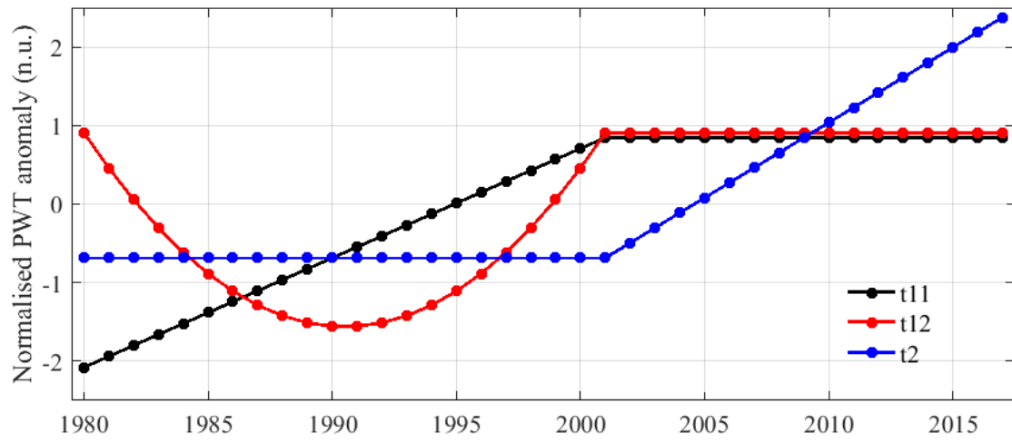
Figure 7: Anomalies of the linear functions before and after 2001 (t11 and t2, respectively) and parabolic function (t12) that correspond to the PWT proxy (see Eq. 2 to 5). Each proxy anomaly is normalised by the corresponding standard deviation.
