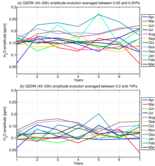
Figure 8. Monthly break down of Q2DW (43–53 h) amplitude development over the 7 investigated years. The \text{H}_2\text{O} amplitudes are pressure layer averaged: 0.05–0.2 hPa (top plot) and 0.2–1 hPa (bottom plot).
