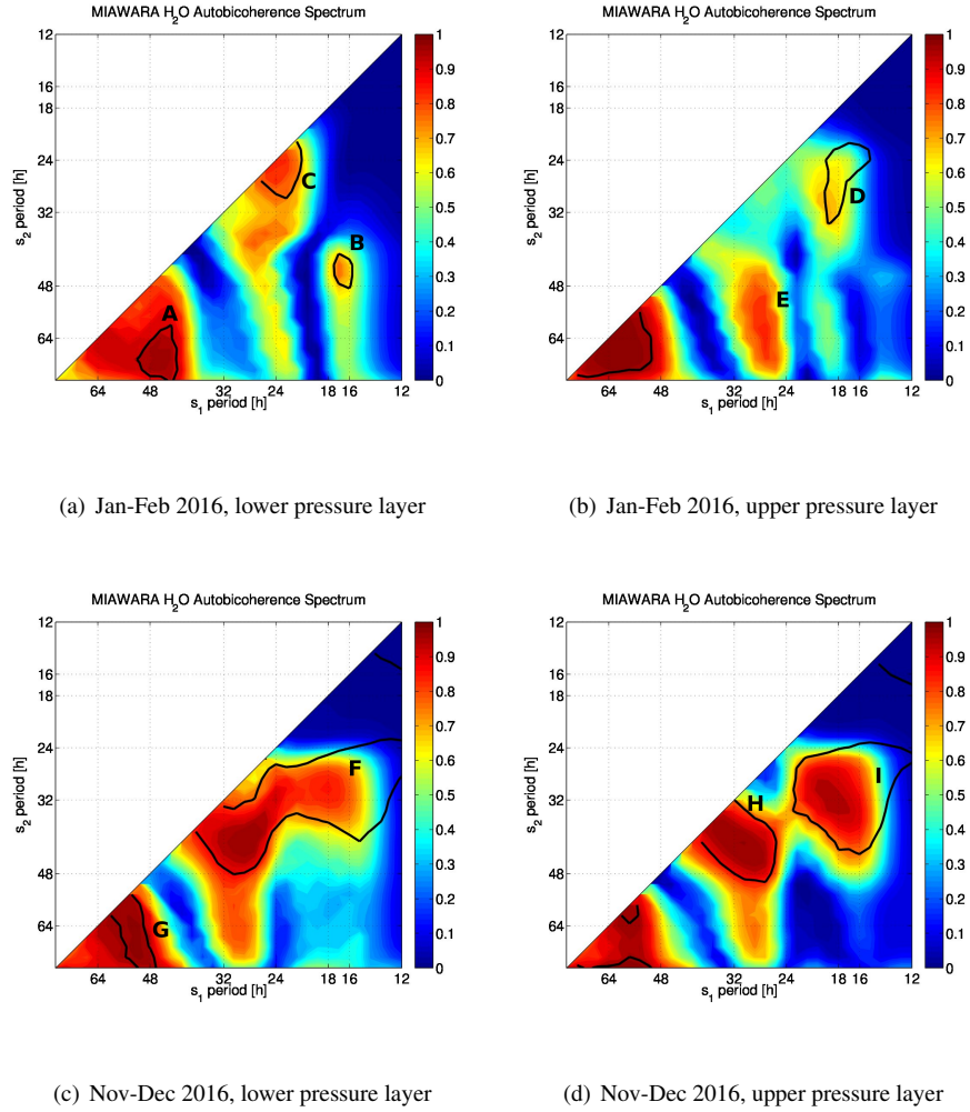
Figure 9. Wavelet-based autobicoherence spectrum from pressure layer averaged MIAWARA water vapor time series with individual lengths of two months. The chosen pressure layers are 0.05–0.2 hPa and 0.2–1 hPa. Thick contours enclose regions of 80 % point-wise confidence after controlling the FDR (False Detection Rate). The diagonal line separates the 2-dimensional spectrum into two symmetric regions. Interesting features on the plots are labeled with capital letters (A–H).
