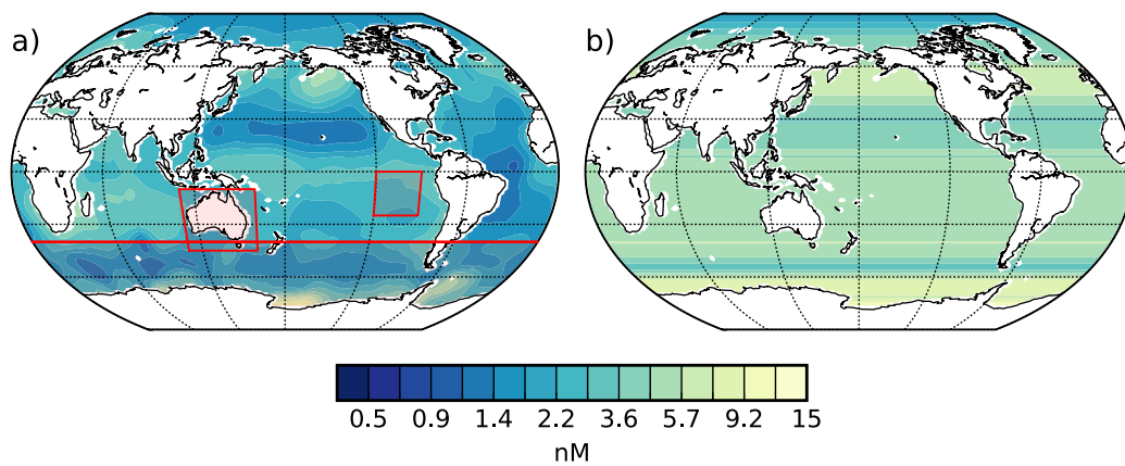
Figure 2. The annual mean concentrations of a) the Lana et al. (2011) DMS w climatology, b) the DMS w field of the second experimental run: zonal maximum DMS w . Additionally, three regions of interest are shown in a) by red boxes, the Australian region: 45^{\circ}S - 10^{\circ}S , 110^{\circ}E - 160^{\circ}E , the South
