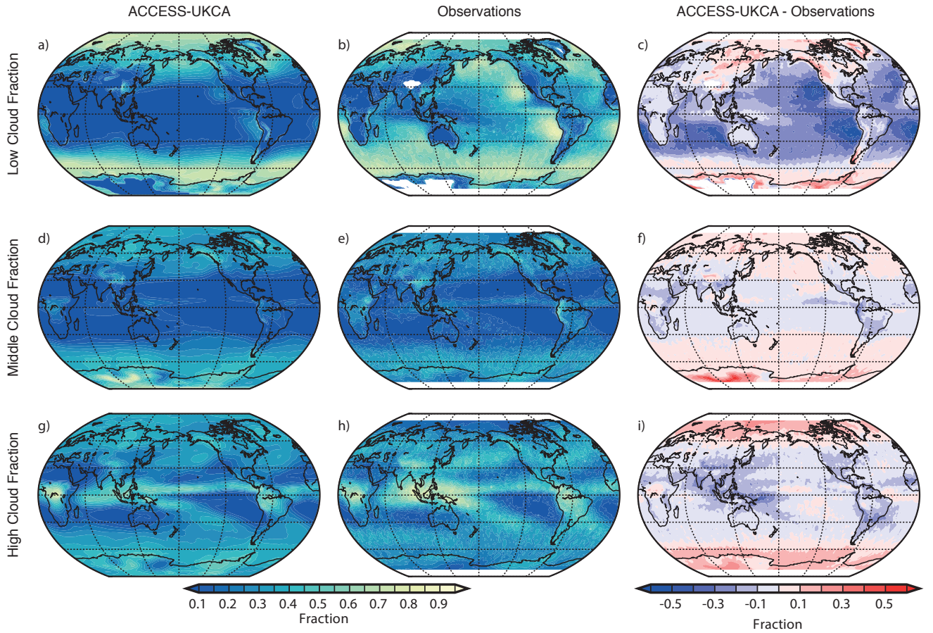
Figure 3. The 2006-2009 annual mean of the ACCESS-UKCA CTL-Ctl (first column) compared to the CALIPSO-GOCCP (Chepfer et al., 2010) climatology (second column), with the absolute -relative differences between the two shown in the third column ( model - observations ). The top row shows the low cloud fraction, the middle row shows the middle cloud fraction and the bottom row the high cloud fraction
