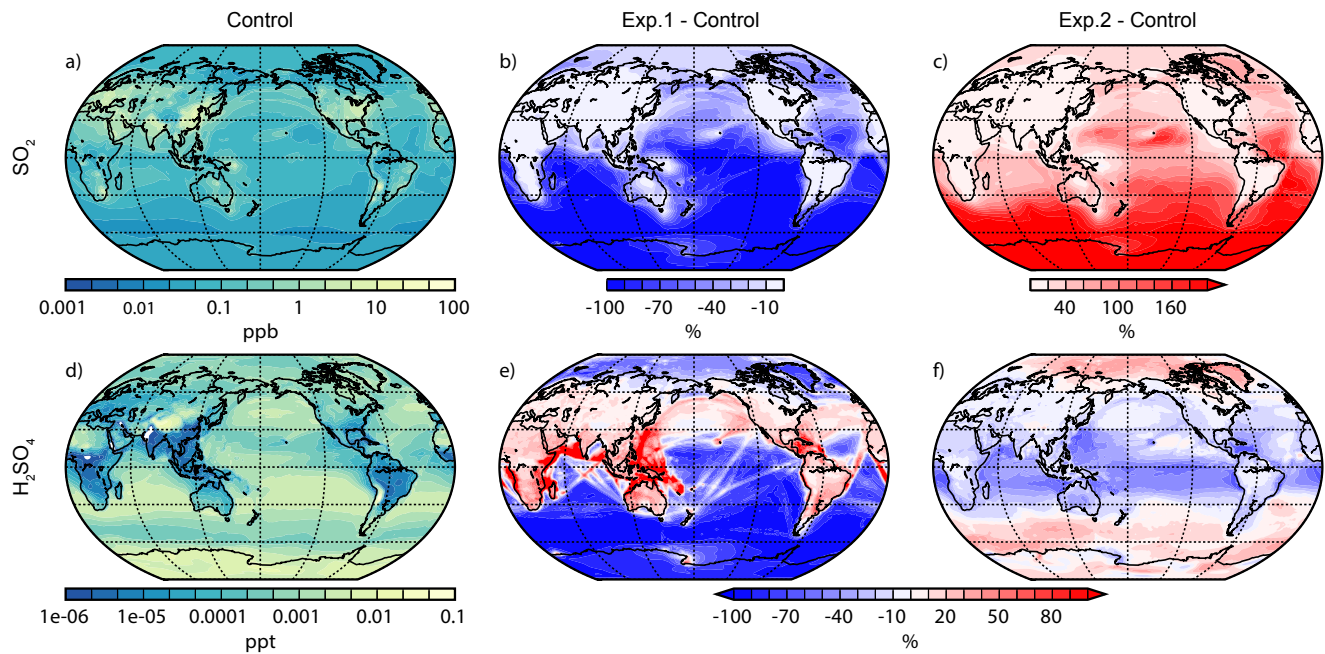
Figure 6. Mean (2000-2009) values for the Ctl (first column), the difference between Exp.1 (zero DMS w ) and the Ctl (second column) and the difference between Exp.2 (zonally enhanced DMS w ) and the Ctl (third column). The first row shows the volume mixing ratio of SO 2 in ppb; the second row the volume mixing ratio of H 2 SO 4 in ppt
