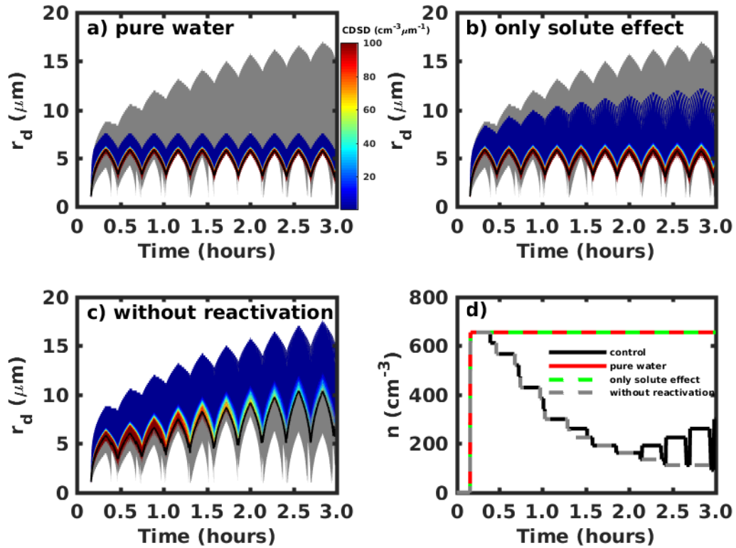
Figure 3. a) Cloud droplet size distribution (CDS) changes with time without solute or curvature effects. b) CDS changes with time with the solute effect but without the curvature effect. c) CDS changes with time including both solute and curvature effects but where droplet reactivation is not considered. d) Total cloud droplet number concentration ( n ) changes with time for the different cases. The gray region in a-c represents the range of the droplet size spectrum for the control case, and the black lines represent the mean cloud droplet radius change with time.
