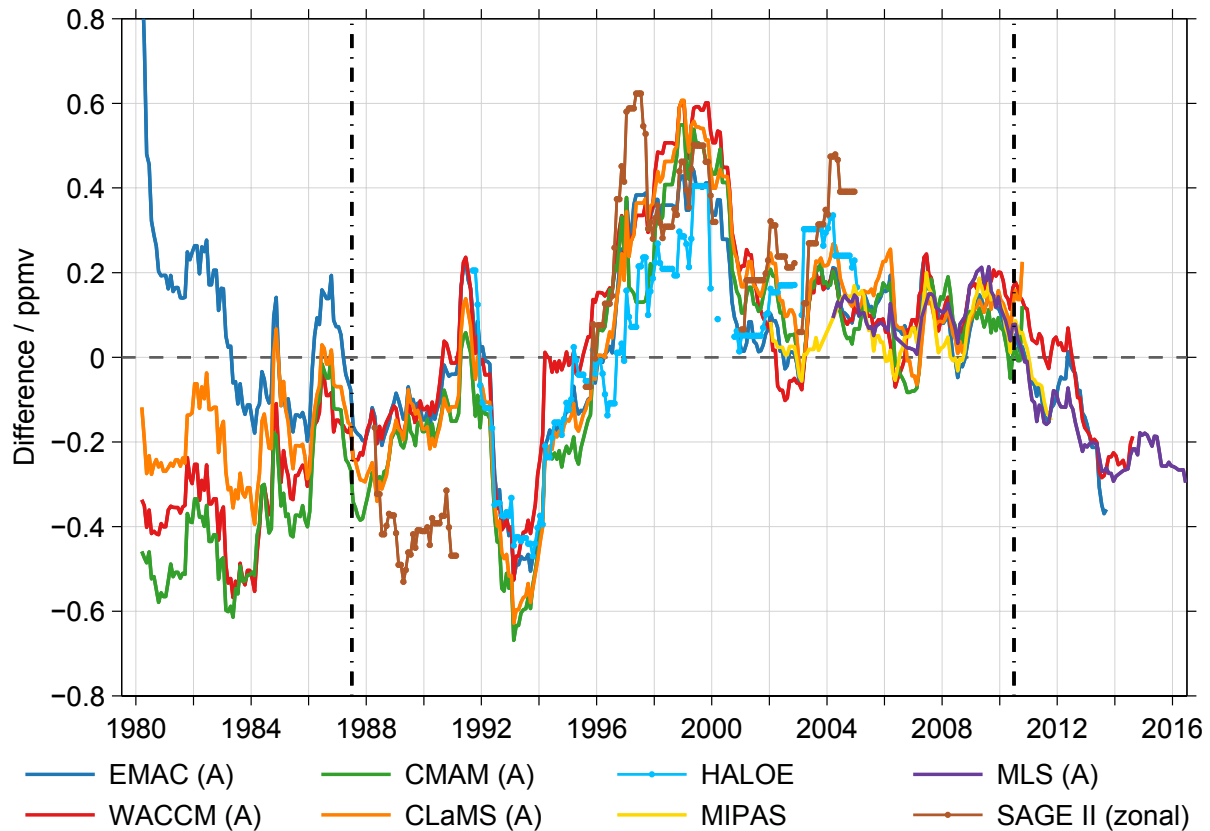
Figure 8. Differences between the de-seasonalised time series obtained from the FPH observations and the Boulder time series derived from the different simulations and observational results at 70 hPa. To provide a clearer picture, the differences are smoothed with a 1 year running average. At least three data points are required for a valid running average. The dashed-dotted line indicates the time period covered by the merged satellite data set at this altitude. The time ticks consider again the middle of the specified years.
