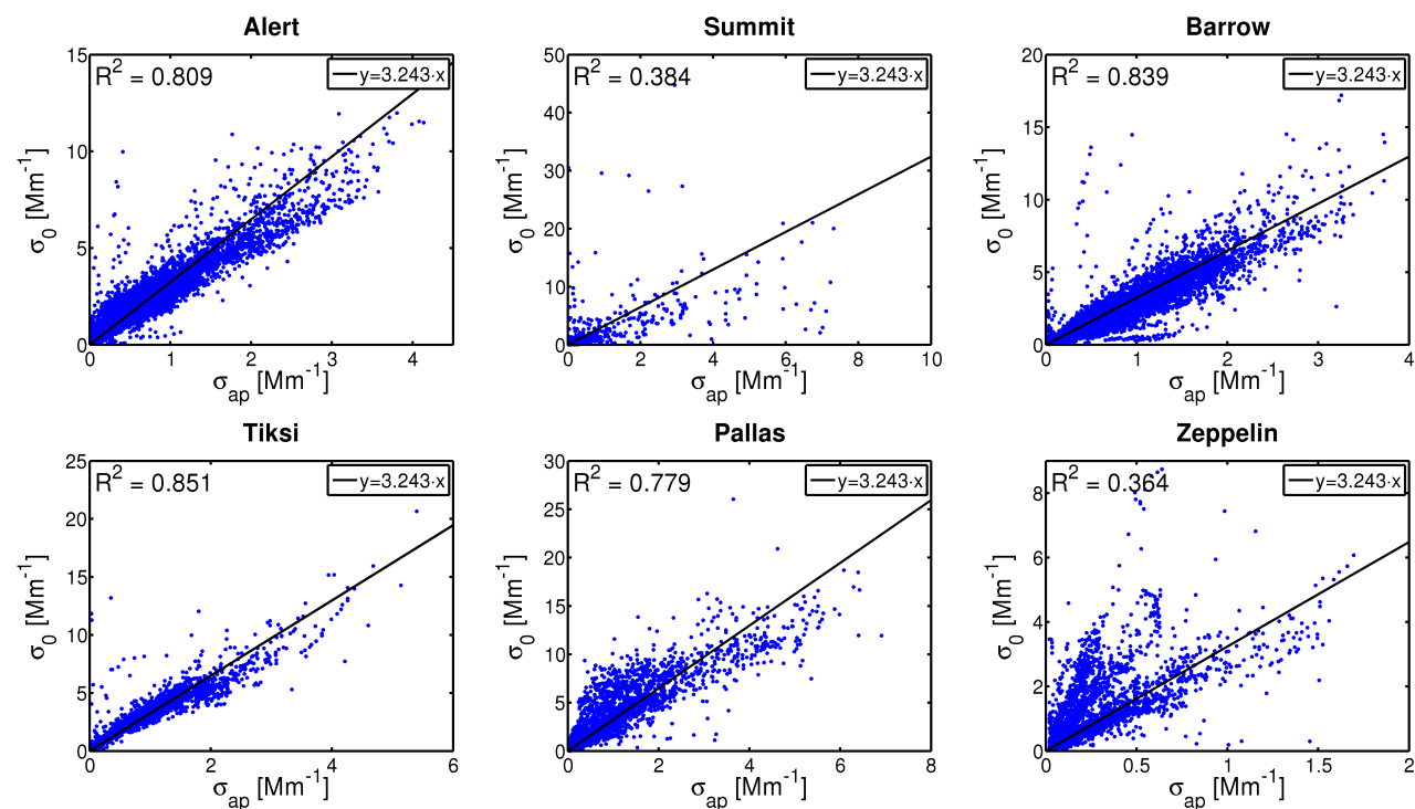
Figure S1. Scatter plots comparing Aethalometer and reference absorption data, \sigma_0 and \sigma_{ap} , respectively, for each of the six Arctic monitoring stations. Regression coefficients are noted in the top left of each plot. A reference line of y=3.243x is shown in black on each plot.
