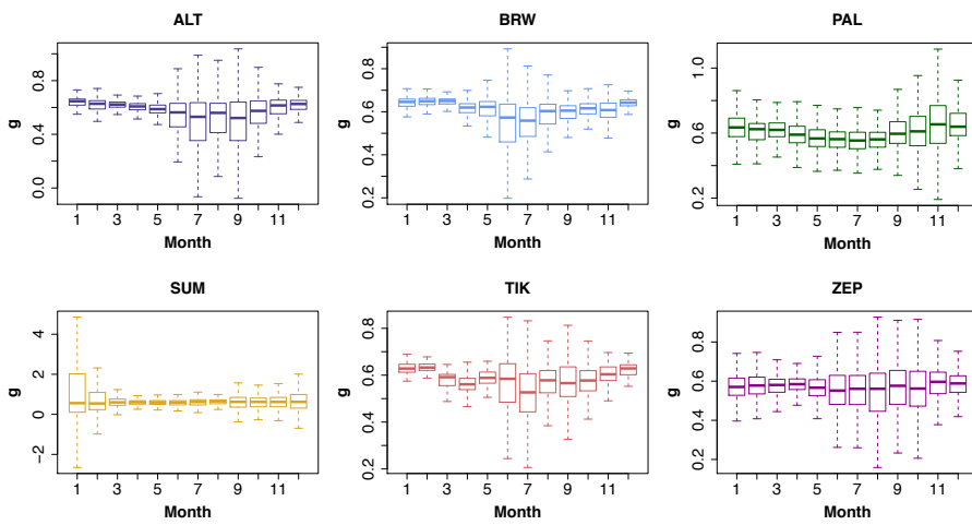
Figure 7. Seasonality of aerosol asymmetry parameter ( g ) at all sites. Large plot shows monthly medians of hourly average g at 550nm at each station, subplots below show boxplots of g at individual sites with horizontal line at the median, edges of the box at 25 th and 75 th percentiles, and whiskers at 5 th and 95 th percentiles. Note that y-axes are difference on each plot.
