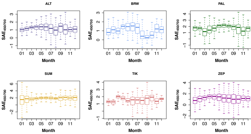
5 Figure 6. Seasonality of scattering Ångström exponent (SAE) at all sites. Large plot shows monthly medians of hourly average SAE at the 450nm/700nm wavelength pair at each station, subplots below show boxplots of SAE at individual sites with horizontal line at the median, edges of the box at 25 th and 75 th percentiles, and whiskers at 5 th and 95 th percentiles. Note that y-axes are different on each plot.
