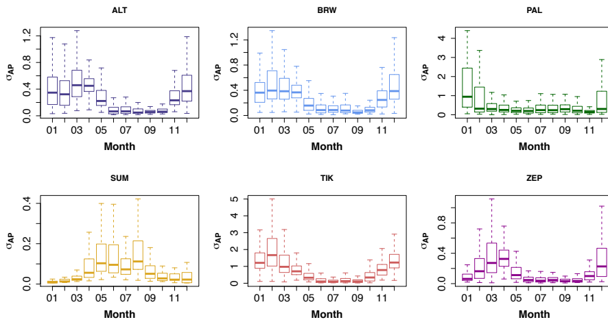
Figure 4. Seasonality of aerosol light absorption coefficient ( \sigma_{ap} ) at 550nm at all sites. Large plot shows monthly medians of absorption in Mm^{-1} at each station, subplots below show boxplots of hourly average absorption at individual sites with horizontal line at the median, edges of the box at 25 th and 75 th percentiles, and whiskers at 5 th and 95 th percentiles. Note that y-axes are different on each plot. Size cuts for the Aethalometer absorption measurements are as follows: 10 \mu m (ALT), 2.5 \mu m (SUM), 10 \mu m (TIK) and no size cut at BRW, PAL, and ZEP.
