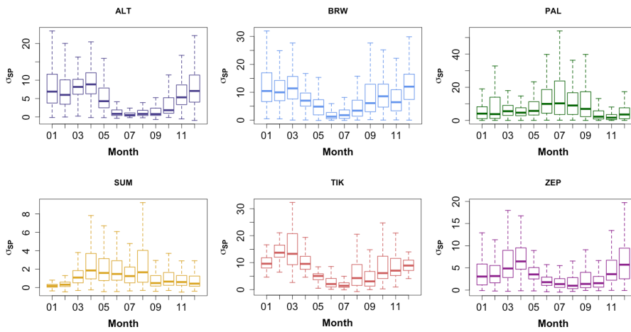
Figure 3. Seasonality of aerosol light scattering coefficient ( \sigma_{sp} ) at 550nm at all sites. Large plot shows monthly medians of scattering in Mm^{-1} at each station, subplots below show boxplots of hourly average scattering at individual sites with horizontal line at the median, edges of the box at 25 th and 75 th percentiles, and whiskers at 5 th and 95 th percentiles. Note that y-axes are different on each plot. Size cuts for the scattering measurements are as follows: 10 \mu m (ALT), 10 \mu m (BRW), 10 \mu m (PAL), 2.5 \mu m (SUM), 10 \mu m (TIK) and no size cut at ZEP.
