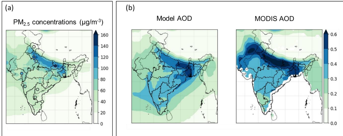
Figure 4. Model Evaluation by (a) comparison of simulated annual mean PM_{2.5} concentrations with in-situ observations (circles = observations) and (b) comparison of modeled annual mean AOD over India with observations from MODIS.
