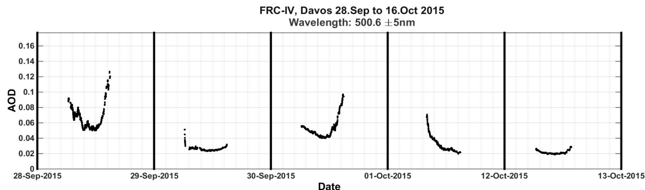
Figure 1: Average AOD at 500 nm measured by the three reference PFR instruments (WORCC-WORCC triad) during 5 days with cloud free sky conditions. The symbols represent 1-minute measurements.
