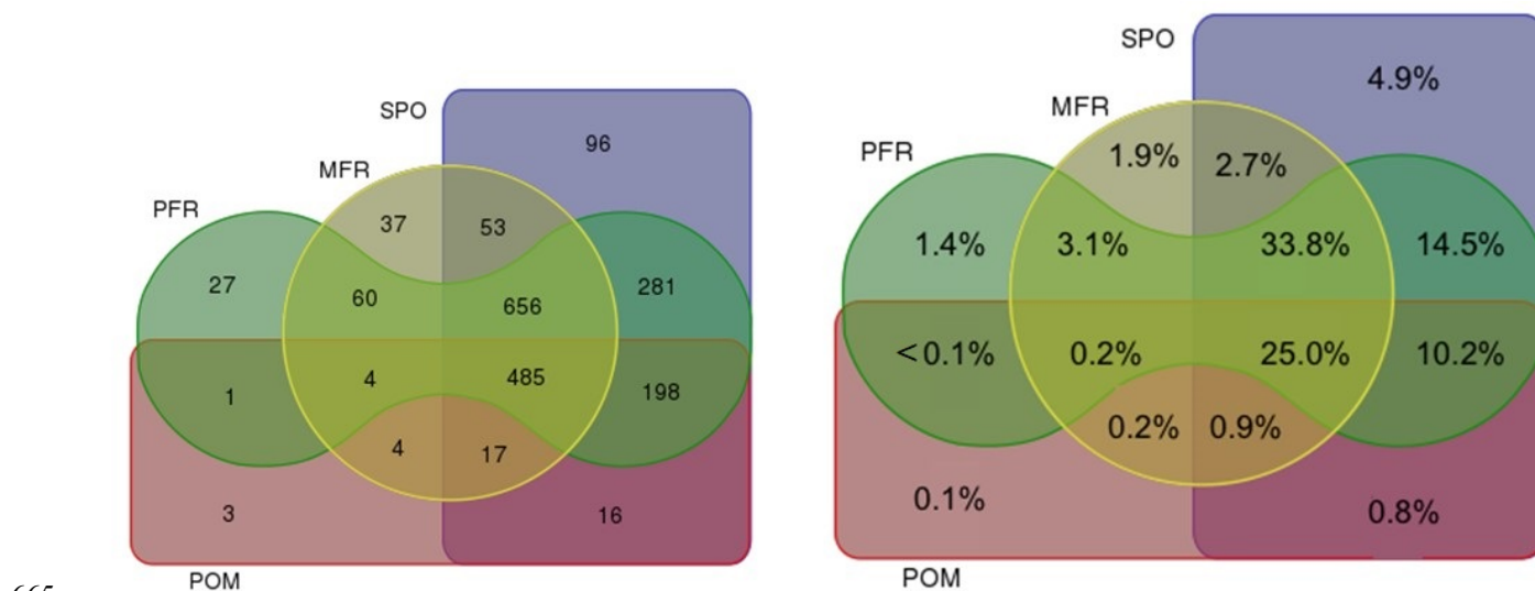
Figure 7: Venn diagram of quality controlled, clear sky data sets of SPO, MFR, PFR, and POM data for four cloudless ( only very limited presence of clouds ) days. Left panel: number of measurements, right panel: percentage of measurements.
