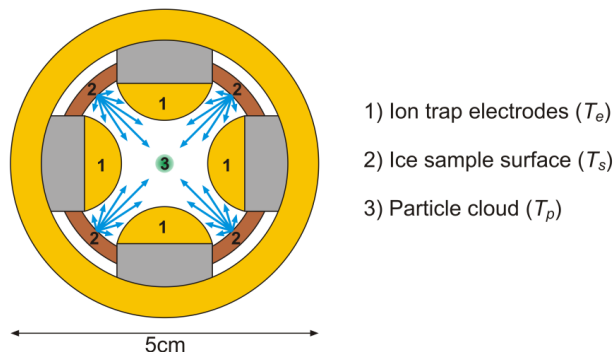
Figure 1: Radial cross section of MICE.
