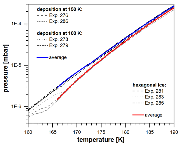
Figure B2: Vapor pressure between 160 K and 190 K after deposition at 100 K and 150 K (black lines, 4 runs) and after crystallization of hexagonal ice from liquid water at 260 K (grey lines, 3 runs). The solid blue and red lines represent calculated mean values for deposition at 100 K / 150 K and hexagonal ice, respectively.
