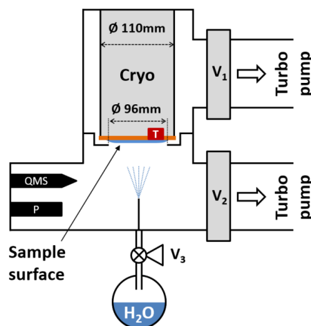
10 Figure B1: Experimental setup used for the relative saturation vapor pressure measurements between 166 K and 190 K. A hot-cathode ionization gauge (P) is employed in a vacuum chamber which is evacuated via valves V_1 and V_2 by two turbo molecular pumps. Simultaneous quadrupole mass spectrometer (QMS) measurements ensure that no other trace gases than H_2O bias the pressure readout. See text for details.
