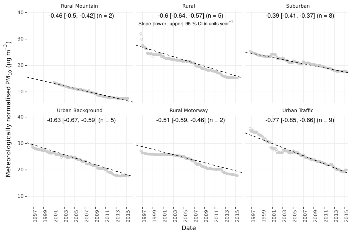
Figure 5. Aggregated meteorologically normalised PM 10 trends for the six site types in Switzerland between 1997 and 2016. Points represent the aggregated meteorologically normalised monthly means, lines represent the trend estimate, and n represents the number of sites in the group.
