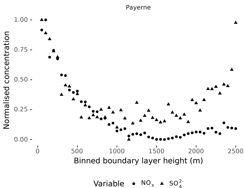
Figure 9. Mean normalised concentrations of \text{SO}_4^{2-} , a secondary PM species and \text{NO}_x for binned boundary layer heights (bin was set at 50 metres) at Payerne between 1997 and 2016.
