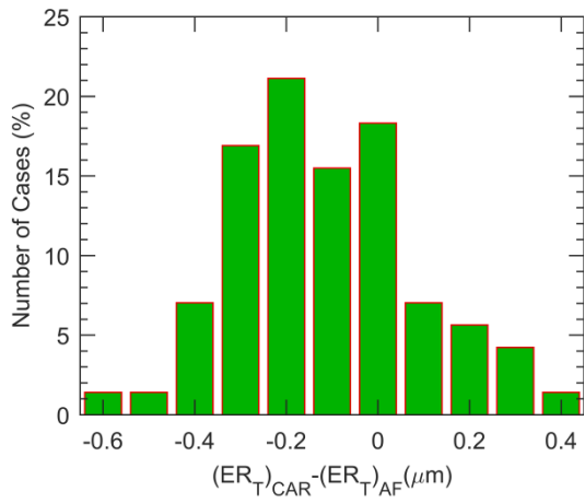
Figure 10: Histogram of the differences between the total effective radii in the African region and in the Caribbean area for those cases with connected desert dust conditions in both areas (“ D_{AF} + D_{CAR} ” case).
