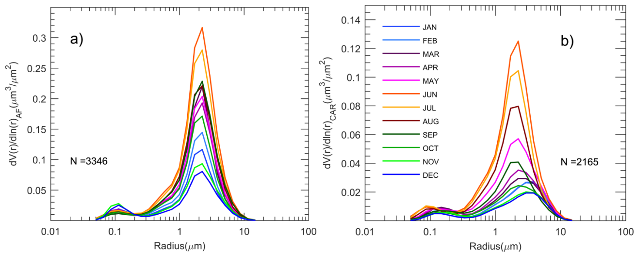
Figure 5: Monthly averages of the volume particle size distribution ( dV(r)/d\ln(r) ) from 1996 to 2014 in West African (a) and Caribbean (b) areas.
