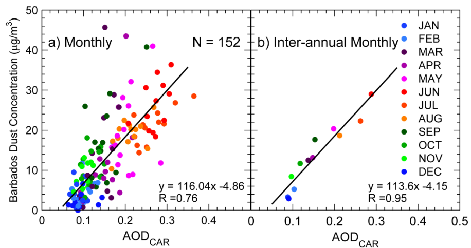
Figure 4: Scatterplot of (a) monthly and (b) inter-annual monthly means of surface dust concentration and AOD in the Caribbean Basin in the period 1996-2011. Solid line indicates the linear fit between both quantities and R indicates the correlation coefficient.
