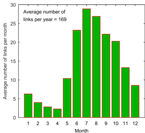
Figure 6. Seasonal cycle of number of Africa-Caribbean Sea air mass connections. The number of air mass links is 169 per year, with a total of 3174 links in the 19-year analyzed period.
