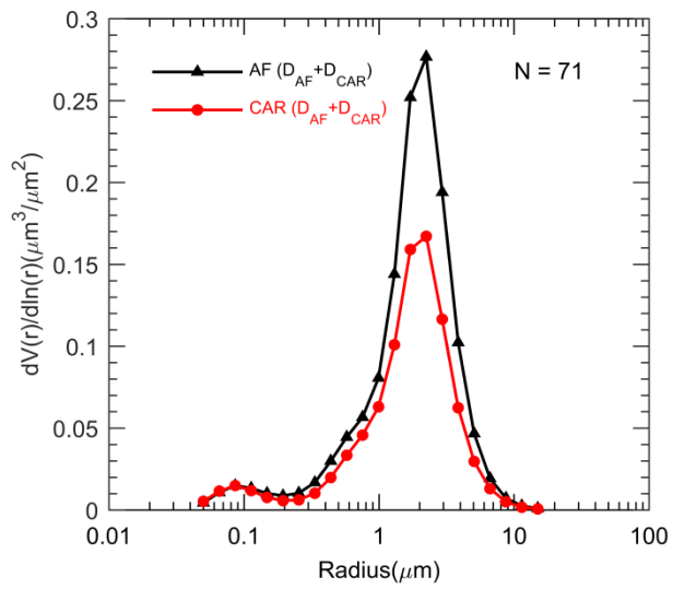
Figure 9: Volume particle size distribution ( dV(r)/d\ln(r) ) in the African (AF) and the Caribbean (CAR) areas under desert dust conditions (“ D_{AF} + D_{CAR} ” case, see Section 2.2).
