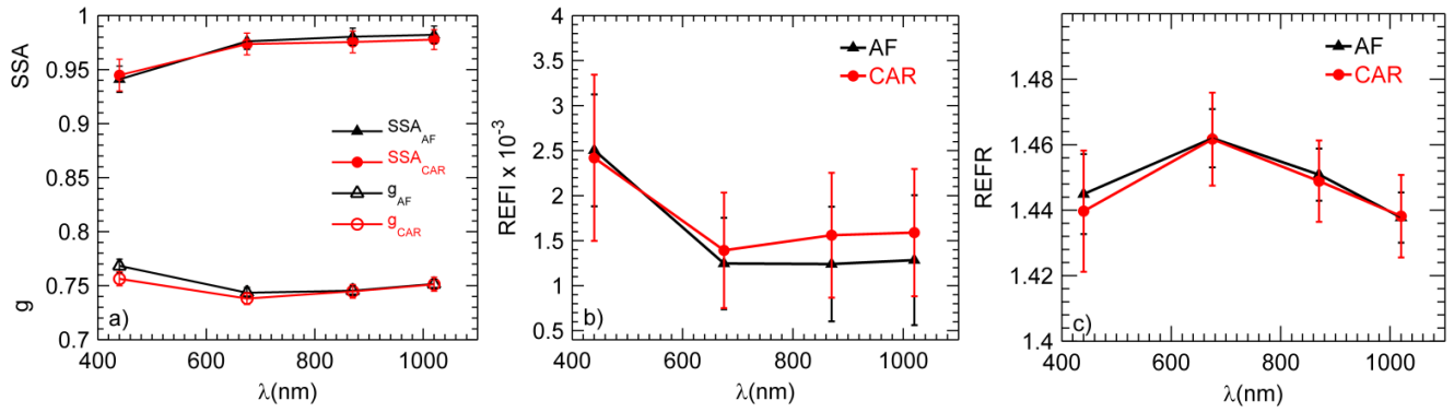
Figure 12: Average values of (a) Single scattering albedo (SSA) and asymmetry parameter ( g ), (b) Imaginary part of the refractive index (REFI), (c) Real part of the refractive index (REFR) for those cases with desert dust in both African region (black lines) and Caribbean area (red lines) ( D_{AF}+D_{CAR} case, see Section 2.2).
