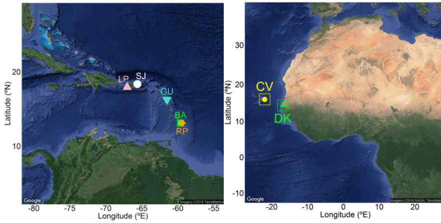
Figure 1: AERONET sites in the Caribbean Zone-area (left) and African zone-region (right). For acronyms see Table 1.
