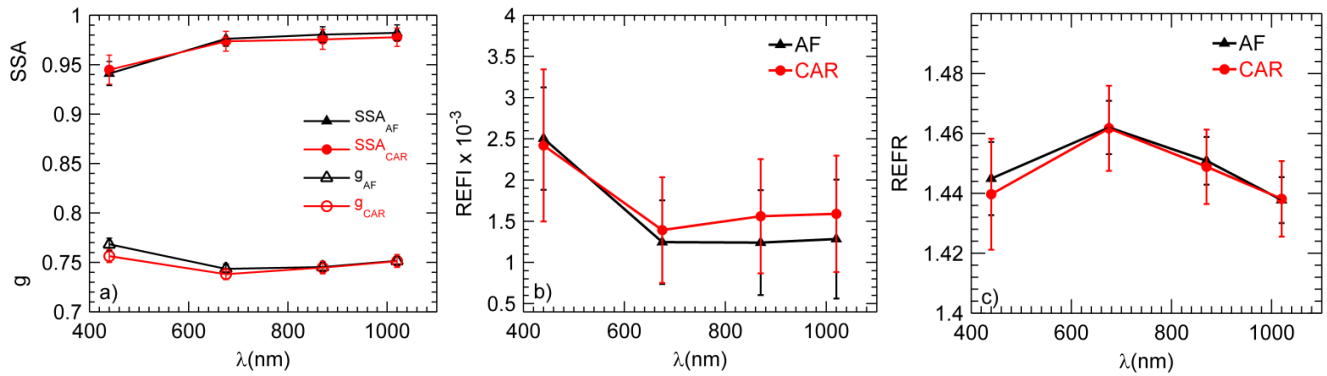
Figure 12: Average values for of (a) Single scattering albedo (SSA) and asymmetry parameter ( g ), (b) Imaginary part of the refractive index (REFI), (c) Real part of the refractive index (REFR) for those cases with desert dust in both African zone-region (black lines) and Caribbean area (red lines) ( D_{AF}+D_{CAR} case, see Section 2.2).
