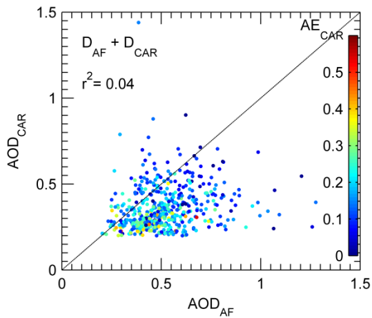
5 | Figure 8. Scatterplot of AOD in the Caribbean ( AOD_{CAR} ) versus AOD in the African zone-region ( AOD_{AF} ) when dust is observed in both areas ( D_{AF}+D_{CAR} case, see Section 2.2). The color scale bar indicates the AE in the Caribbean zone area ( AE_{CAR} ) when dust is observed in both areas ( D_{AF}+D_{CAR} case, see Section 2.2). Solid lines point out indicates no change in AOD data between both areas.
