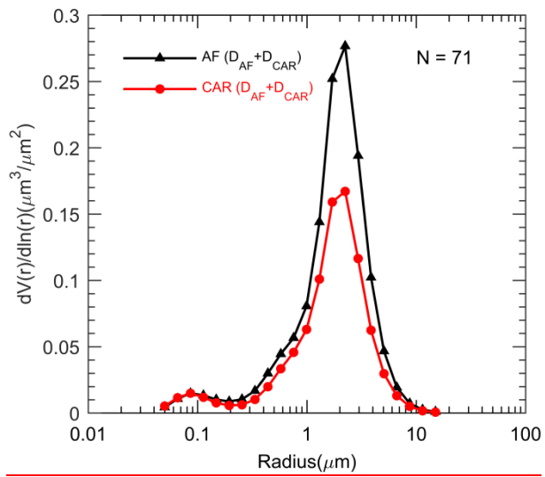
Figure 9: Volume particle size distribution VPSD ( dV(r)/d\ln(r) ) in the African (AF) and the Caribbean (CAR) areas under desert dust conditions (“ D_{AF} + D_{CAR} ” case, see Section 2.2).
