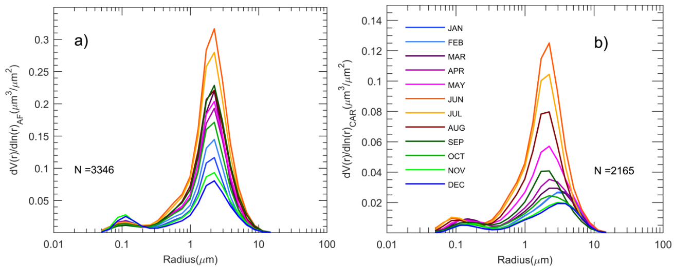
Figure 5: Monthly averages of VPSD the volume particle size distribution ( dV(r)/d\ln(r) ) from 1996 to 2014 in West African (a) and Caribbean (b) areas.
