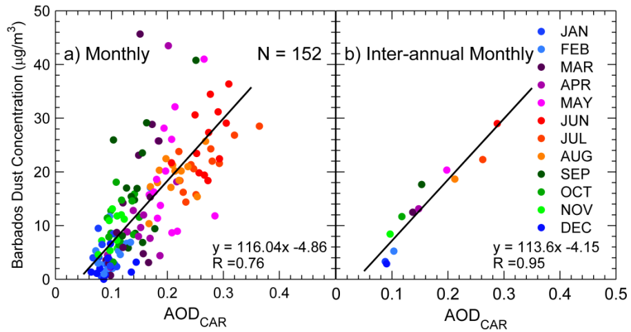
Figure 4: Scatterplot of: (a) monthly and (b) inter-annual monthly means of surface dust concentration and AOD in the Caribbean Basin in the period 1996-2011. Solid line highlights-indicates the linear fit between both quantities.
