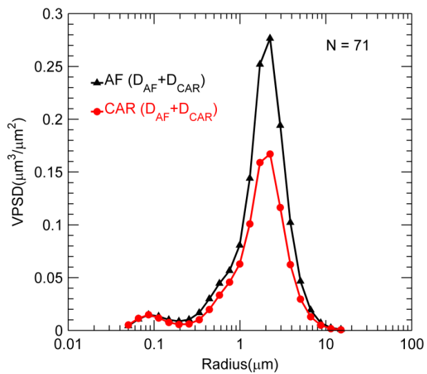
Figure 9: VPSD in the African (AF) and the Caribbean (CAR) areas under desert dust conditions (“ D_{\text{AF}} + D_{\text{CAR}} ” case, see Section 2.2).
