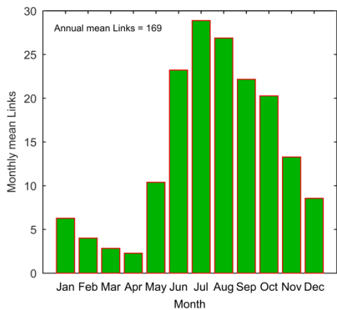
Figure 6. Seasonal cycle of number of Africa-Caribbean Sea air mass connections. The total number of air mass links is 169 per year, with a total of 3174 links in the 19-year analyzed period.
