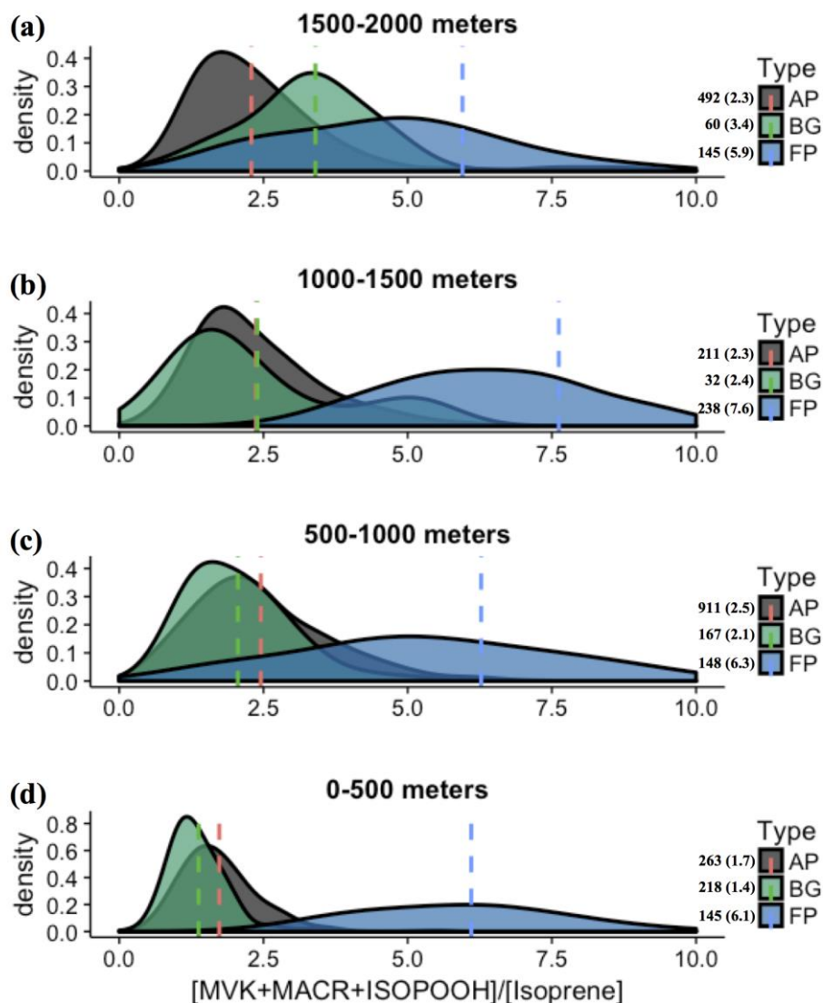
845 Figure 8. Density distributions of the ratio [MVK+MACR+ISOPOOH]/[isoprene] , at the altitude layers (a) 1,500 - 2,000 m, (b) 1,000 - 1,500 m, (c) 500 - 1,000 m and (d) 0 - 500 m. The Kernel analysis was carried out considering the classification for background (BG), aged smoke (AP), and fresh smoke plumes (FP). The number of samples and mean values for each group are depicted near the color bars.
