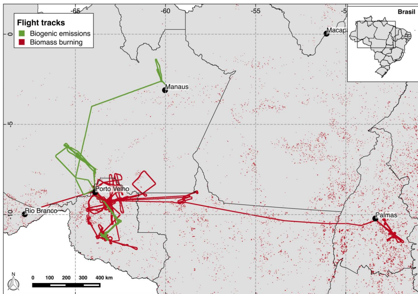
770 Figure 1. SAMBBA flights tracks according to their original goals as biogenic emissions (green) and biomass burning (red). The black dots indicate the locations of the taking-off and landing airports. The red points depict the fires detected by MODIS onboard 775 AQUA satellite during the SAMBBA campaign from 14 September - 3 October 2012.
