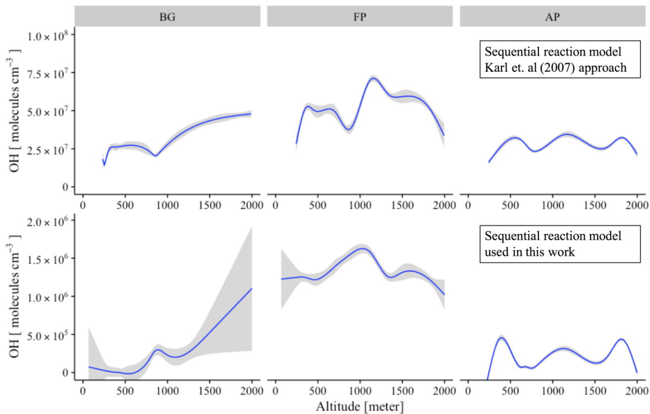
850 Figure 9. Vertical profile of OH concentration (molecules cm -3 ) for the different chemical regimes: background environment (BG), fresh smoke plume (FP), and aged smoke plume (AP). On top, the sequential reaction model according to the original approach of Karl et al. (2007), and on bottom, the new approach used in this work. Blue lines are the trend lines and grey intervals represents the level of confidence (0.95) used.
