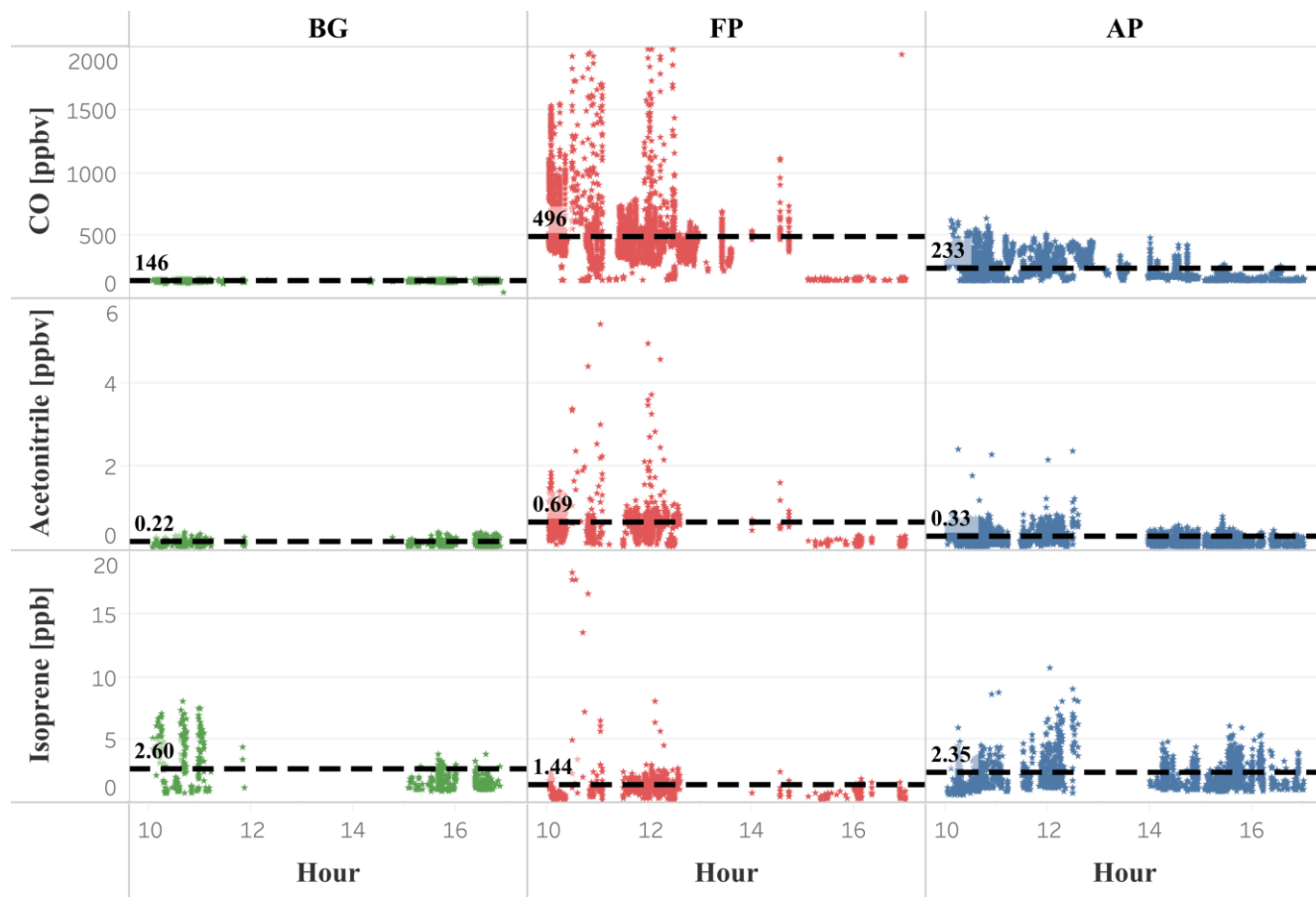
830 Figure 6. Isoprene, Acetonitrile and CO mixing ratios (ppbv) as function of daytime (local time) for the different chemical regimes previously classified as background (green dots), fresh smoke plume (red dots), and aged smoke plume (blue dots). Black dashed lines, and the numbers next to them, represent the mean values of the measurements taken below 2,000 m altitude. Hour is presented in local time (11:00 – 18:00 h).
