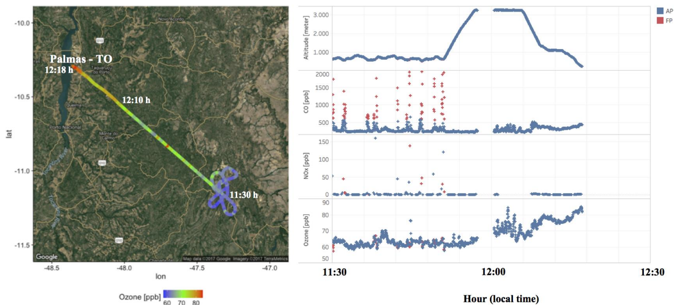
800 Figure 4. On the left, the track of flight B742 that landed in Palmas – TO. The color bar represents the measured O 3 mixing ratios (ppbv) along the flight track. On the right, from top to bottom, the altitude, and the CO, NO x and O 3 mixing ratios (ppbv) measured along the B742 flight track. The red and blue dots represent the parts of the flight track classified as fresh (FP) and aged (AP) smoke plumes, respectively.
