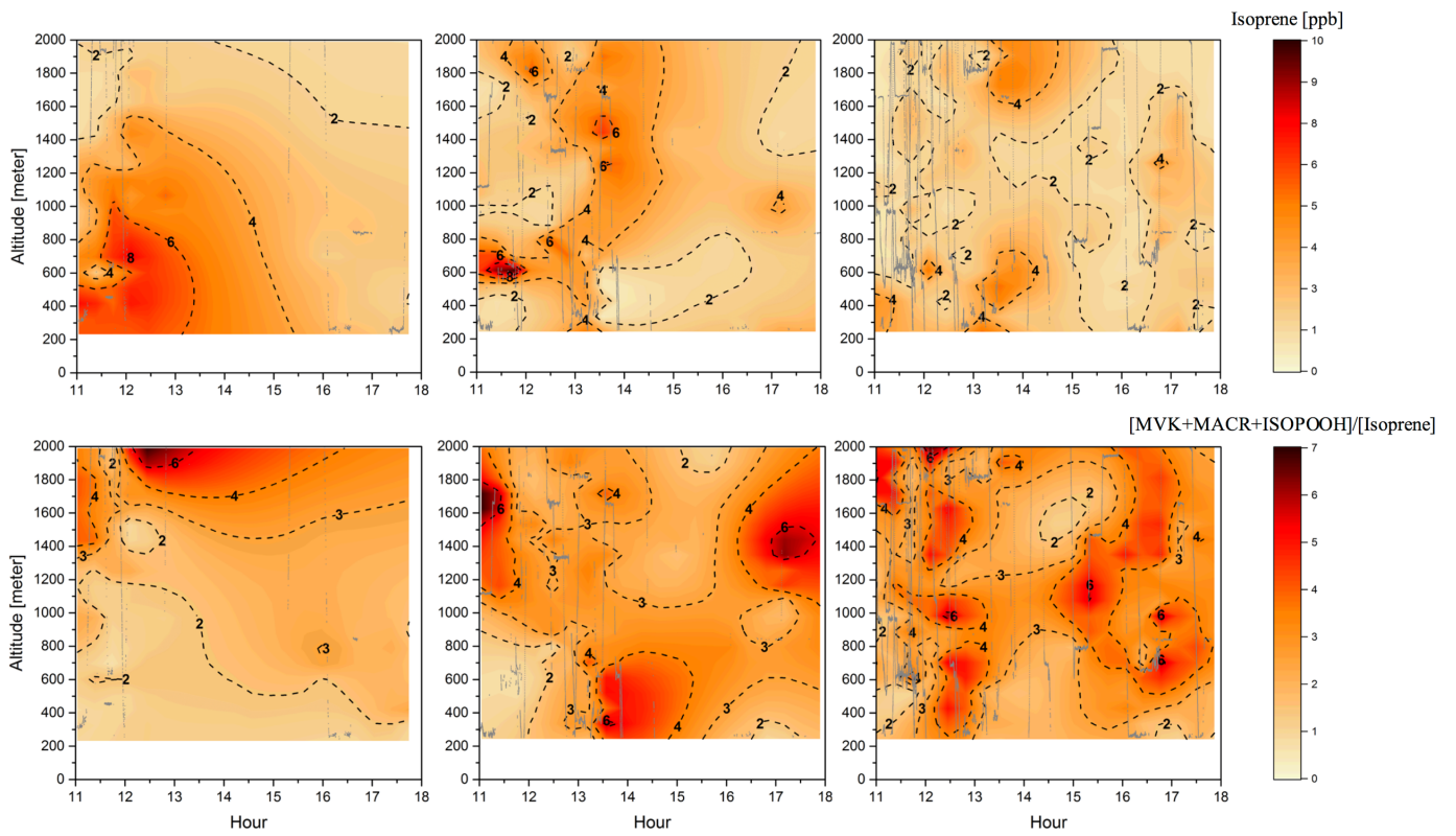
820 Figure 5. Cross-section of the isoprene mixing ratio (ppbv) (top) and the [MVK+MACR+ISOPOOH]/[Isoprene] ratio (bottom) for the three different groups: background environment (on the left), fresh smoke plume ( t < 2 hours, in the middle), and aged smoke plume ( t > 2 hours, on the right). The aircraft data were interpolated from the various vertical profile measurements using kriging correlation method. White dashed lines show the flight tracks. Hour is presented in local time.
