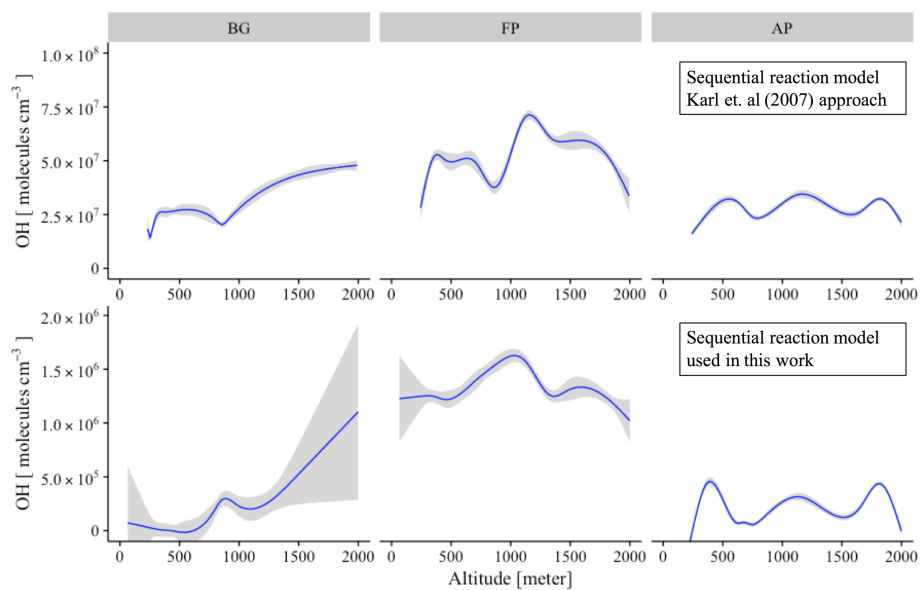
Figure 9. Vertical profile of OH concentration (molecules \text{cm}^{-3} ) for the different chemical regimes: background environment (BG), fresh smoke plume (FP), and aged smoke plume (AP). On top, the sequential reaction model according to the original approach of Karl et al. (2007), and on bottom, the new approach used in this work. Blue lines are the trend lines and grey intervals represents the level of confidence (0.95) used.
