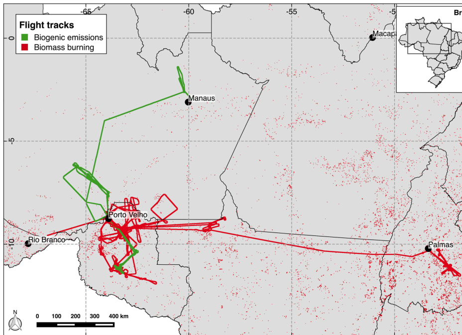
825 Figure 1. SAMBBA flights tracks according to their original goals as biogenic emissions (green) and biomass burning (red). The 830 black dots indicate the locations of the taking-off and landing airports. The red points depict the fires detected by MODIS onboard 835 AQUA satellite during the SAMBBA campaign from 14 September - 3 October 2012.
