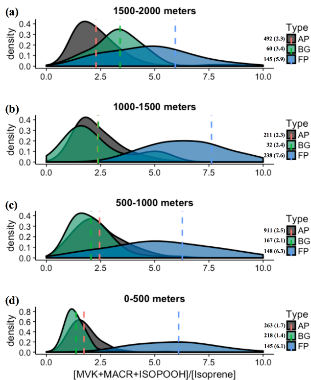
Figure 8. Density distributions of the ratio \frac{[MVK+MACR+ISOPOOH]}{[isoprene]} , at the altitude layers (a) 1,500 - 2,000 m, (b) 1,000 - 1,500 m, (c) 500 - 1,000 m and (d) 0 - 500 m. The Kernel analysis was carried out considering the classification for background (BG), aged smoke (AP), and fresh smoke plumes (FP). The number of samples and mean values for each group are depicted near the color bars.
