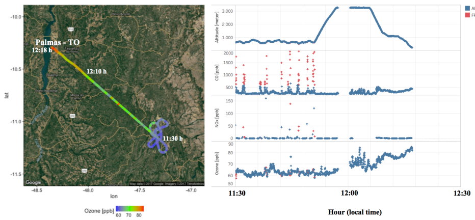
855 Figure 4. On the left, the track of flight B742 that landed in Palmas – TO. The color bar represents the measured O 3 mixing ratios (ppbv) along the flight track. On the right, from top to bottom, the altitude, and the CO, NO x and O 3 mixing ratios (ppbv) measured along the B742 flight track. The red and blue dots represent the parts of the flight track classified as fresh (FP) and aged (AP) smoke plumes, respectively.
