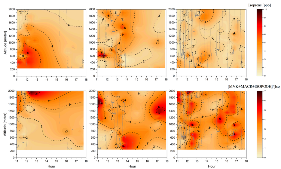
875 Figure 5. Cross-section of the isoprene mixing ratio (ppbv) (top) and the [MVK+MACR+ISOPOOH]/[Isoprene] ratio (bottom) for the three different groups: background environment (on the left), fresh smoke plume ( t < 2 hours, in the middle), and aged smoke plume ( t > 2 hours, on the right). The aircraft data were interpolated from the various vertical profile measurements using kriging correlation method. White dashed lines show the flight tracks. Hour is presented in local time.
