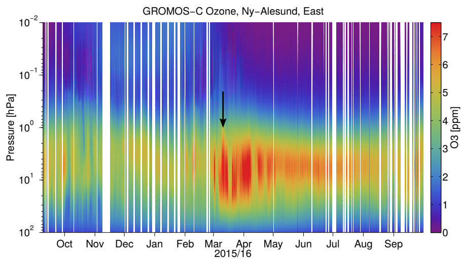
Figure 3. Time series of ozone volume mixing ratio measured by GROMOS-C in eastward direction at Ny-Ålesund. The arrow indicates the sudden stratospheric final warming of March 2016.
