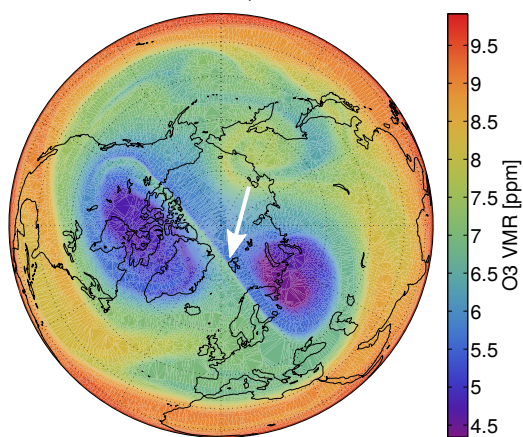
ECMWF Ozone at 10 hPa, 2016-11-02 06:00
