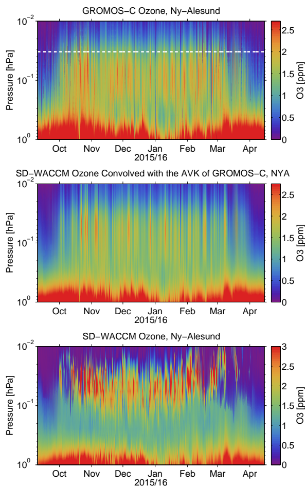
Figure 15. The tertiary ozone maximum at Ny-Ålesund measured by the ground based microwave radiometer GROMOS-C (top). The dashed white line indicates the measurement response of 0.8. Simulation of the tertiary ozone maximum by SD-WACCM convolved with the averaging kernels of GROMOS-C (middle) and unconvolved (bottom).
