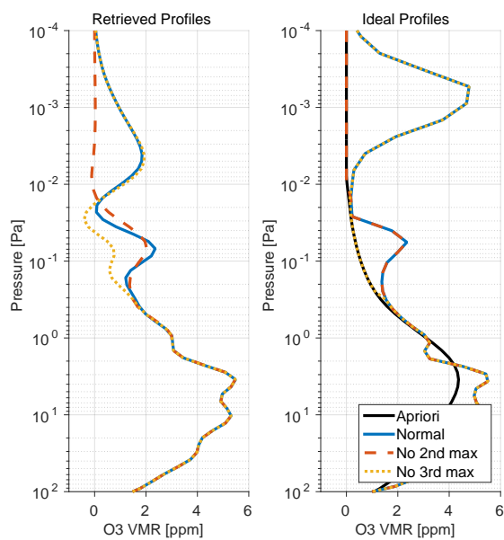
Figure 16. Ozone profiles (left) retrieved from spectra generated with ARTS using different ideal profiles (right). The ideal profile is from SD-WACCM and shows the three ozone maxima. It was modified to have no 2nd or no 3rd maximum.
