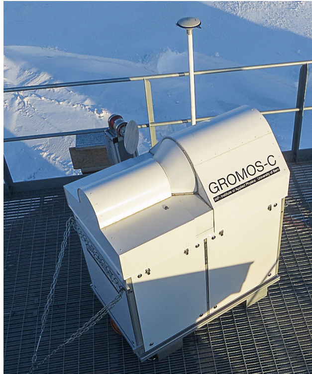
Figure 1. The ground based microwave radiometer GROMOS-C at the AWIPEV research base at Ny-Ålesund, Svalbard (79° N, 12° E). Observations in East and West direction are performed through a conical Teflon window with a rotating mirror inside the housing. North and Southward observations are performed via an external rotating mirror.
