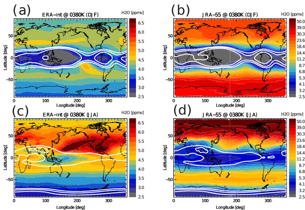
Figure 17. Seasonal mean water vapour distribution averaged over the period from 2004 to 2013 at the potential temperature level of 380 K; DJF indicates winter (a, b), and JJA summer periods (c, d). Shown data are from both reanalysis, ERA-Interim and JRA-55 reanalysis data. The white lines are constant temperature levels from corresponding reanalysis datasets (191 K, 193 K, 195 K). Note the logarithmic colorbar for JRA-55.
