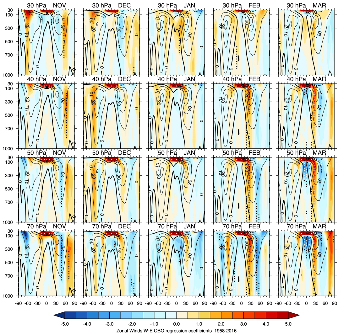
5 Figure 6: As figure 4 but using a linear height scale between 30-1000 hPa to emphasise the tropospheric response. Note the colour scale has been amended accordingly.
