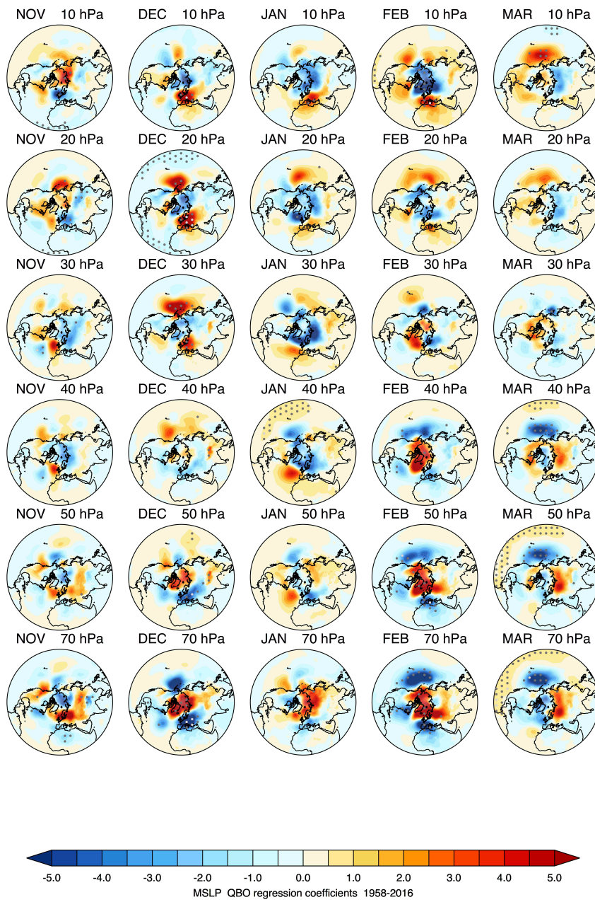
Figure 8: As figure 7 but with an additional index included in the regression analysis to represent the polar vortex variations.
