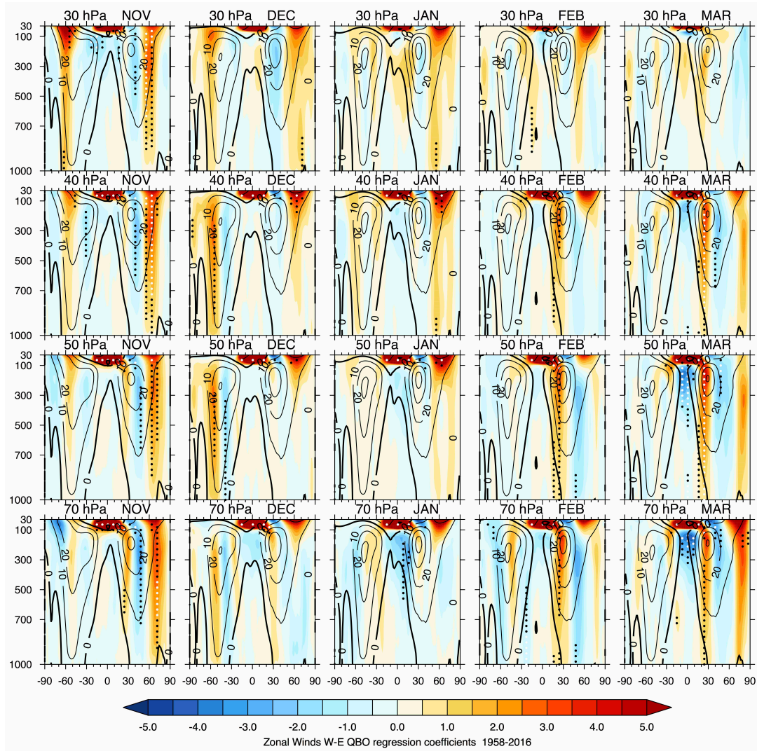
5 Figure 5: As figure 3 but using a linear height scale between 30-1000 hPa to emphasise the tropospheric response. Note the colour scale has been amended accordingly and results are shown for U_{eq}=30-70 hPa only, for brevity.
