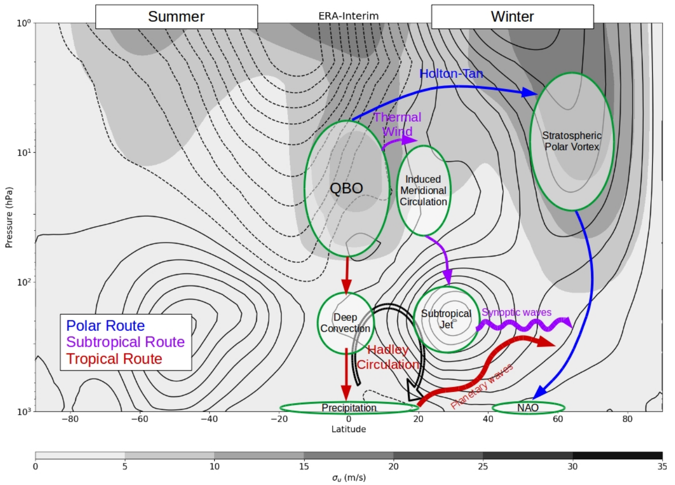
Figure 1. Schematic summarising the three primary routes (tropical, subtropical, polar) for QBO influence at the Earth's surface. Contours show the December-January-February averaged, zonally-averaged zonal winds for 1979-2016 from ERA-Interim data. Contour interval is 5 \text{ ms}^{-1} ; solid contours denote westerlies, dashed contours denote easterlies. Grayscale shows standard deviation of the zonal winds in \text{ms}^{-1} .
