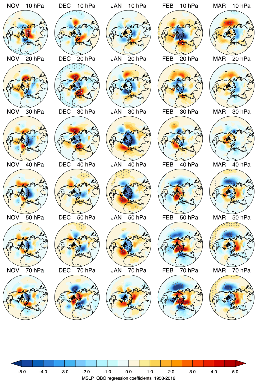
5 Figure 7: Regression based QBO-W minus QBO-E differences: latitude-longitude distribution of mean sea level pressure (hPa) for November – March (columns) from the period 1958-2016. The rows show results for the QBO defined by equatorial zonal wind time-series U_{eq} at different pressure levels from 10 hPa to 70 hPa. White (black) dots indicate 99% (95%) statistical significance.
