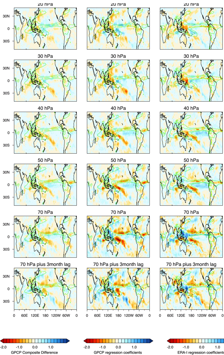
5 Figure 9: Left column: latitude – longitude distributions of annual-averaged W-E QBO composite differences in precipitation (mm per day) using the GPCP dataset for 1979-2016. Middle column: corresponding regression analysis of the GPCP dataset for 1979-2016. Right column: corresponding regression analysis of total precipitation data from the ERA-I dataset for 1979-2016. The rows show results for the QBO defined by the equatorial zonal wind time-series U_{eq} at different pressure levels from 20 hPa to 70 hPa.
