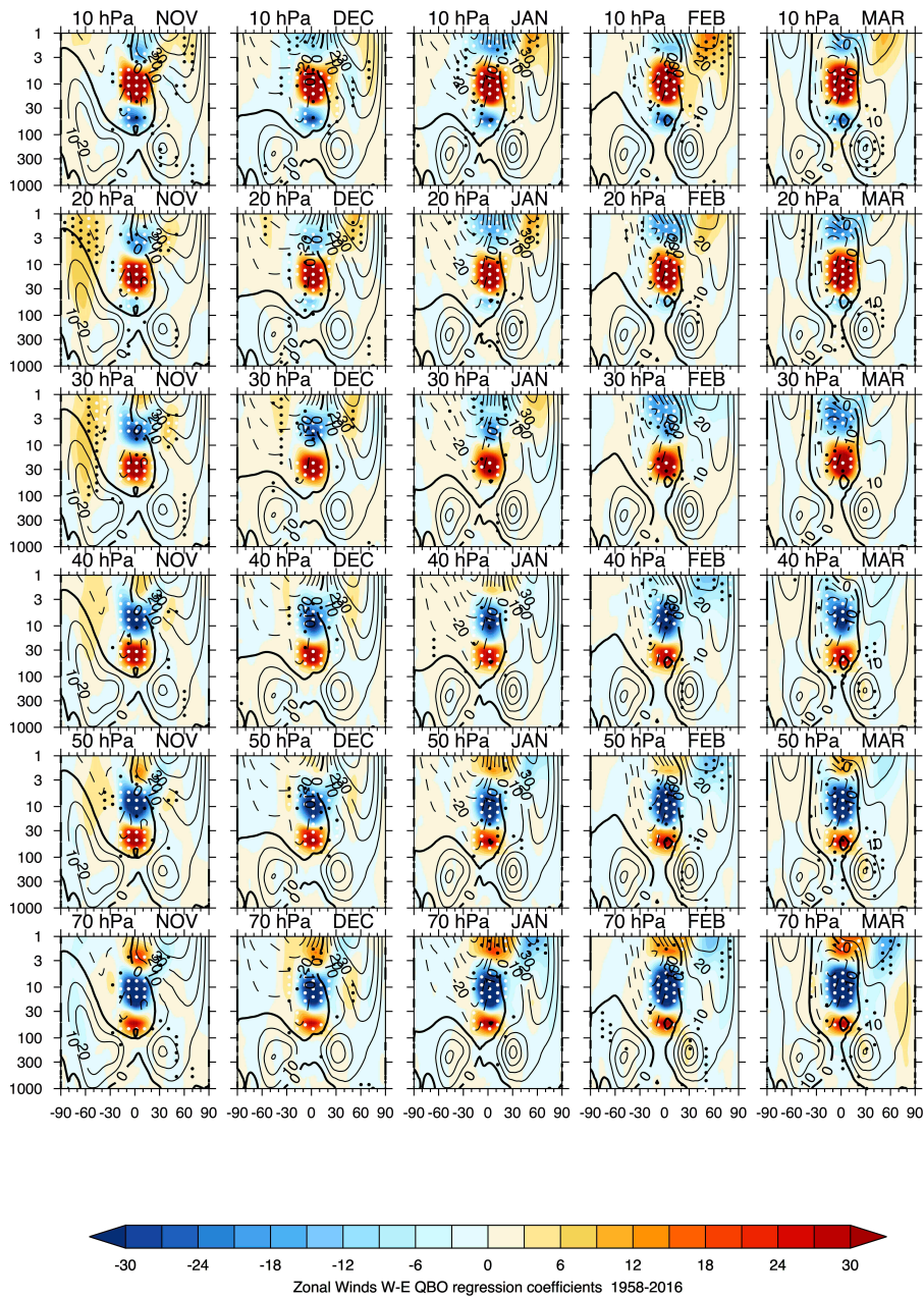
Figure 4: As figure 3 but with an additional index included in the regression analysis to represent the polar vortex variations.
