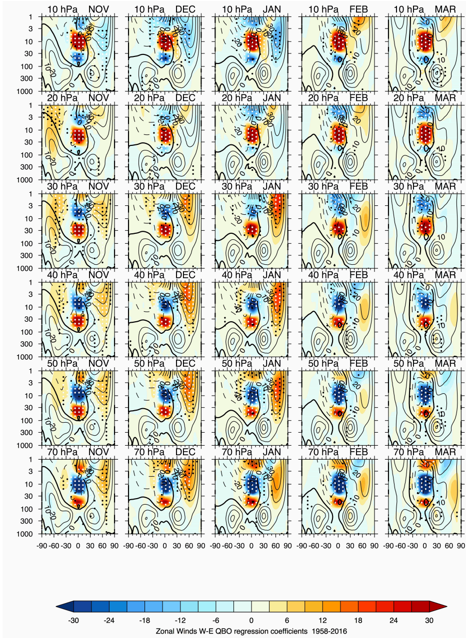
5 Figure 3: Regression based QBO-W minus QBO-E differences: height – latitude cross-sections of zonally-averaged zonal winds ( \text{ms}^{-1} ) for November – March (columns) from the period 1958-2016. The rows show results for the QBO defined by equatorial zonal wind time-series U_{\text{eq}} at different pressure levels from 10 hPa to 70 hPa. Contours show the climatological values (interval of 10 \text{ ms}^{-1} and thick line is the zero value). White (black) dots indicate 99% (95%) statistical significance.
