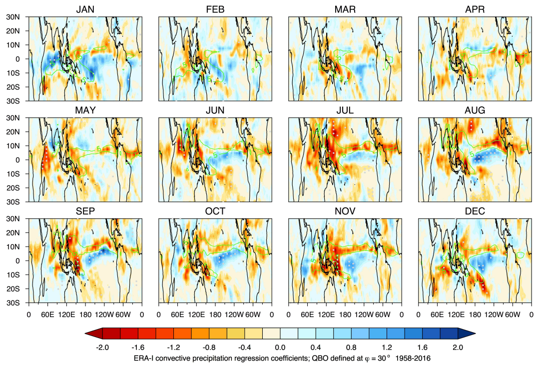
Figure 11: As figure 10 but using \phi = +30^\circ , which is approximately equivalent to defining the QBO by U_{eq} = 30 hPa.
