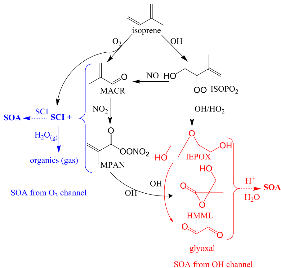
Figure 14: Mechanisms for SOA formation from the O 3 and OH oxidation channels of isoprene.
