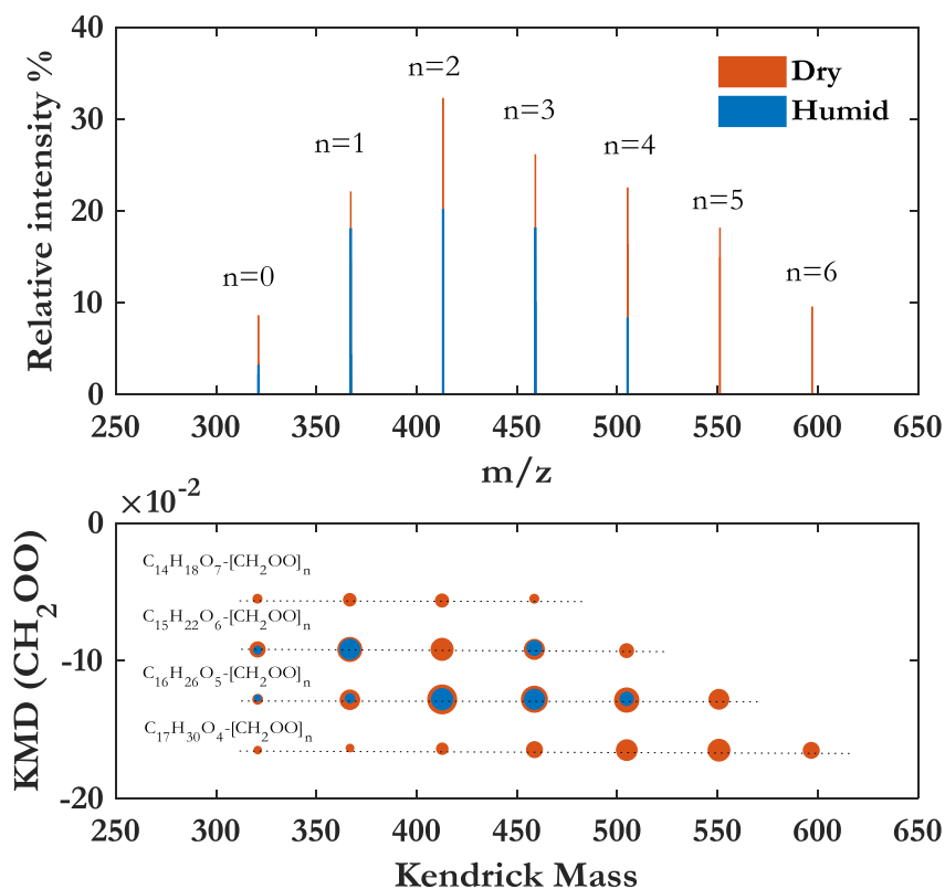
Figure 11: Positive mode mass spectra of oligomers with CH 2 OO as chain units in SOA from isoprene-NO 2 irritations under dry and humid conditions ( top ) and corresponding plots of KMD(CH 2 OO) versus nominal KM(CH 2 OO) ( bottom ). Horizontal lines connect the family of compounds with an equal elemental composition differing only by a [CH 2 OO] n groups (n=0,1,2,3...).
