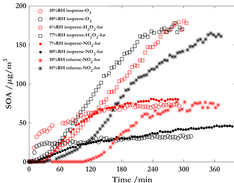
Figure 2: Mass concentration time profiles of SOA from different toluene and isoprene reaction systems under dry and humid conditions. An SOA density of 1.4 \text{ g/cm}^3 was used and applied to the SMPS mass correction (Dommen et al., 2006; Sato et al., 2007). The wall loss rate constant of particles was less dependent on RH conditions, so an average value 4.8 \times 10^{-3} / \text{min} was used to correct the SOA formation.
