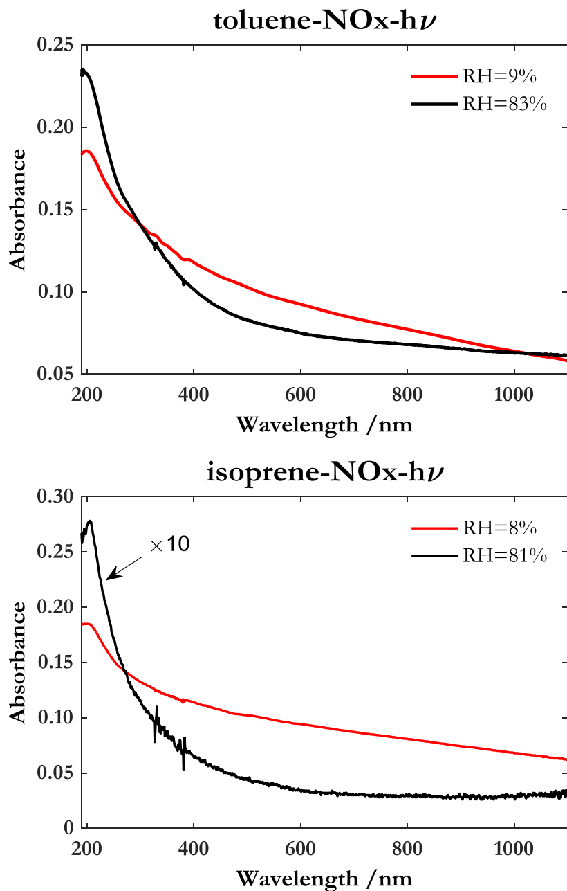
Figure 4: UV-Vis spectra of SOA from toluene and isoprene photooxidations under dry and humid condition.
