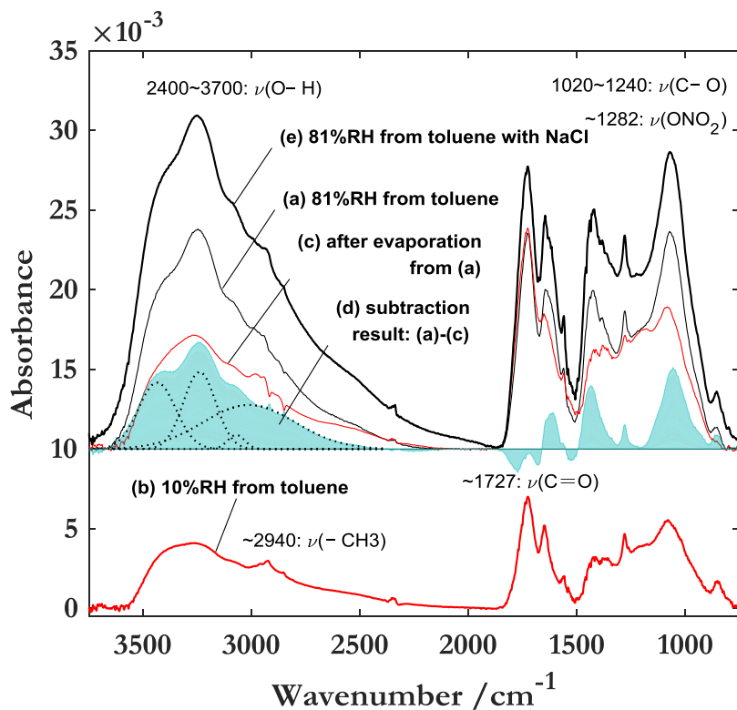
5 Figure 5: The infrared spectra of SOA from toluene irradiations under humid (top: a) and dry (bottom: b) conditions; the infrared spectrum of (c) was obtained after evaporation of SOA from (a) for 15 min at 110 °C; the difference spectrum between (a) and (c) is in blue area (d); the infrared spectrum of (e) is with extra LWC by NaCl seeds. Main bands are hydrogen bonded O–H stretch in alcohols or acids (2400–3700 \text{cm}^{-1} ), the carbonyl (C=O) band at 1727 \text{cm}^{-1} , the organic nitrous (ONO 2 ) bands at 1636, 1278, and 855 \text{cm}^{-1} , the C–OH bend band at 1423 \text{cm}^{-1} , and the C–OH stretch at 1080 \text{cm}^{-1} .
