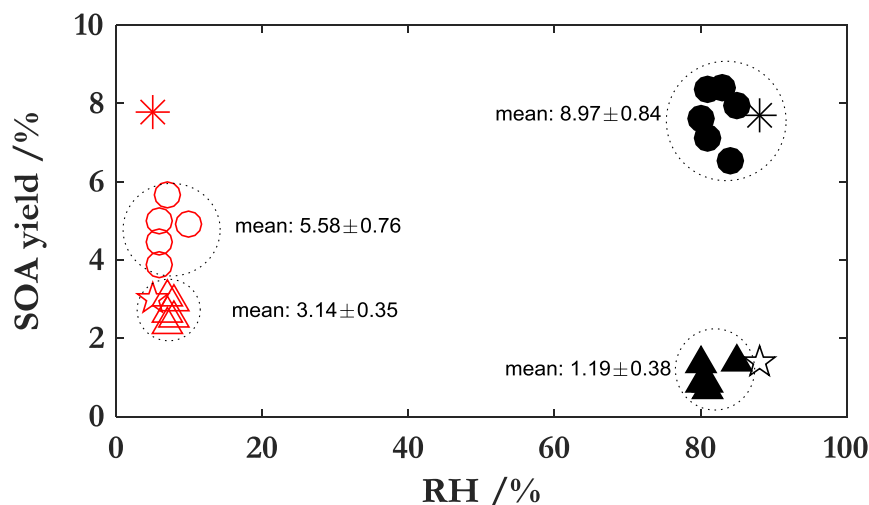
Figure 3: Maximum yields of SOA from toluene and isoprene under dry (red color) and humid (black color) conditions (○: toluene- \text{NO}_2 -h \nu ; Δ: isoprene- \text{NO}_2 -h \nu ; ☆: isoprene- \text{O}_3 ; *: isoprene- \text{H}_2\text{O}_2 -h \nu ).
