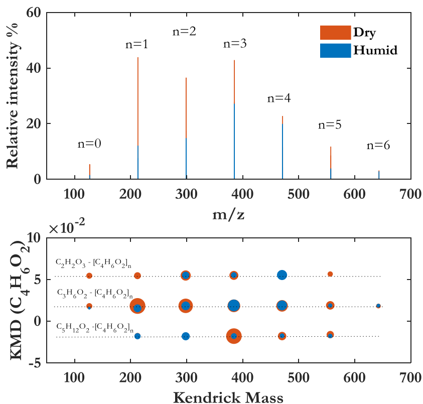
Figure 12: The mass spectra of oligomer with C 4 H 6 O 2 (MACROO and MVKOO) as repeating unit and their Kendrick plots using C 4 H 6 O 2 as Kendrick base. Species separated by C 4 H 6 O 2 groups fall on horizontal lines.
