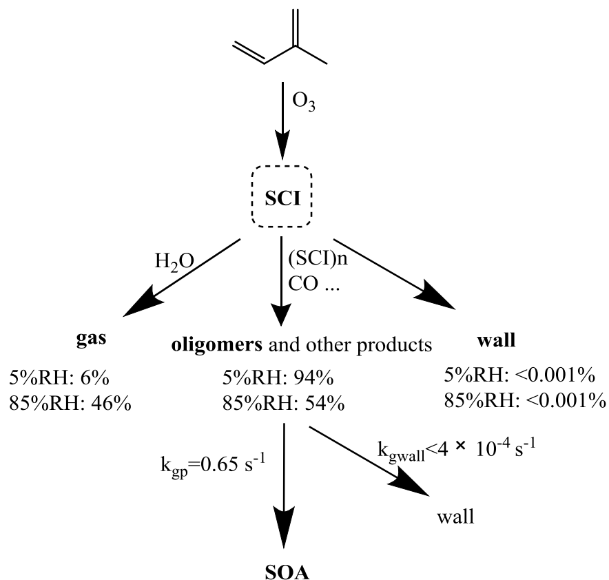
Figure 13: Wall losses vs gas-phase reaction between H_2O and SCI
