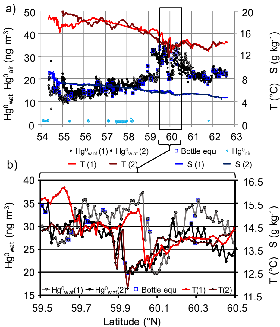
Figure 3: Hg 0 concentration, temperature (T), and salinity (S) data obtained from surface water measurements in July 2013 along a northward (grey, red, blue) and southward (black, dark red, dark blue) transect, respectively. (a) Data for the whole campaign and (b) Hg 0 wat and temperature in the Åland Sea area only. Bottle equilibrator measurements are indicated by blue open squares. Hg 0 atmospheric measurements are given as light blue diamonds in (a) for comparison.
