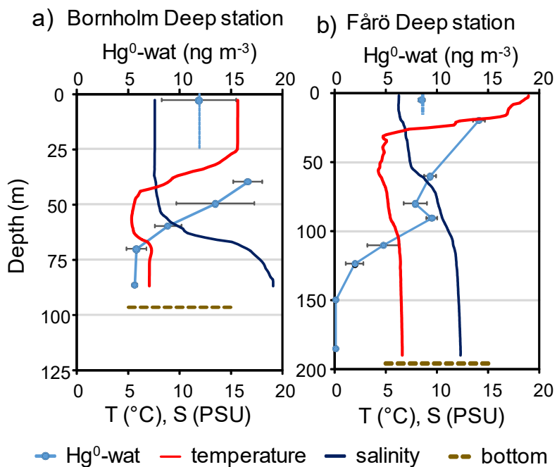
Figure 5: The vertical profiles of Hg 0 , temperature (T), and salinity (S) at the (a) Bornholm Deep and (b) Fårö Deep stations.
