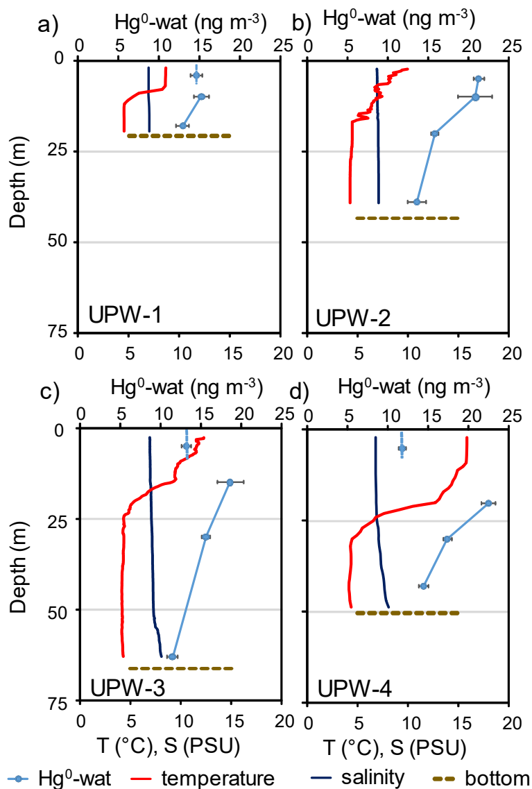
Figure 6: The vertical profiles of Hg^0_{\text{wat}} , temperature (T), and salinity (S) of an upwelling area close to Öland Island (Sweden) measured in 2015. The four stations UPW-1, UPW-2, UPW-3, and UPW-4 were separated by two, one, and six nautical miles, respectively.
