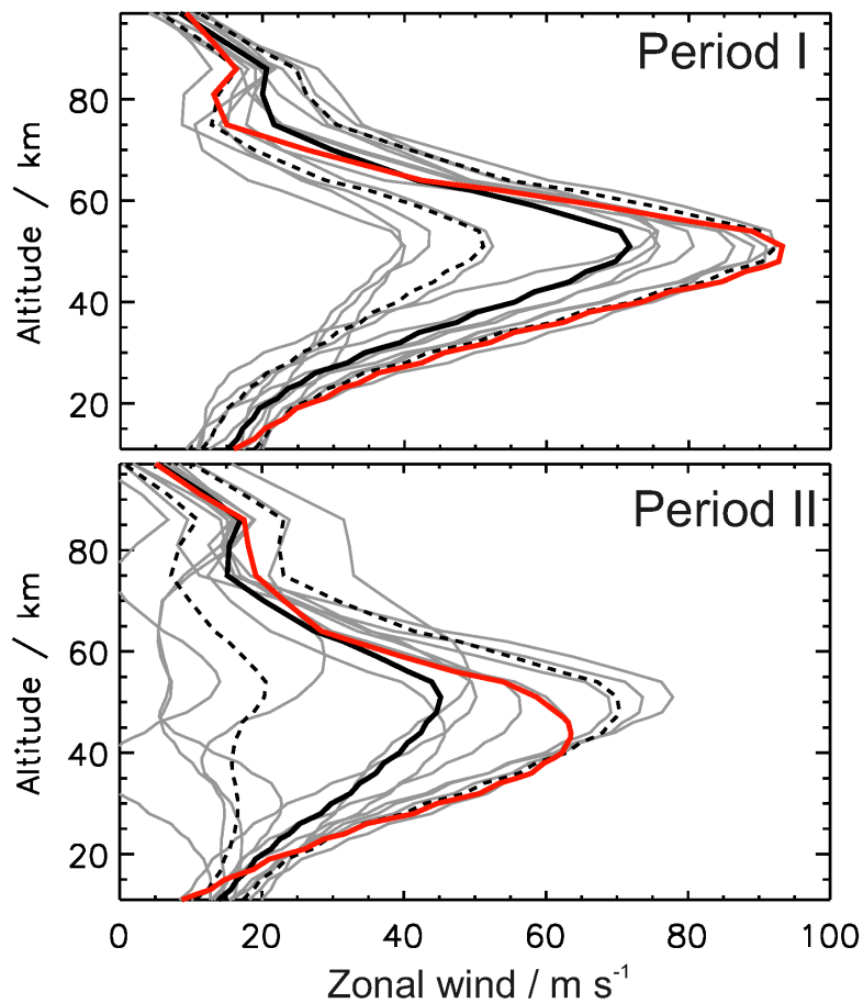
Fig. 1. Profile of the geostrophic zonal wind averaged between 50 and 60°N. Data are derived by MLS GPH data.
