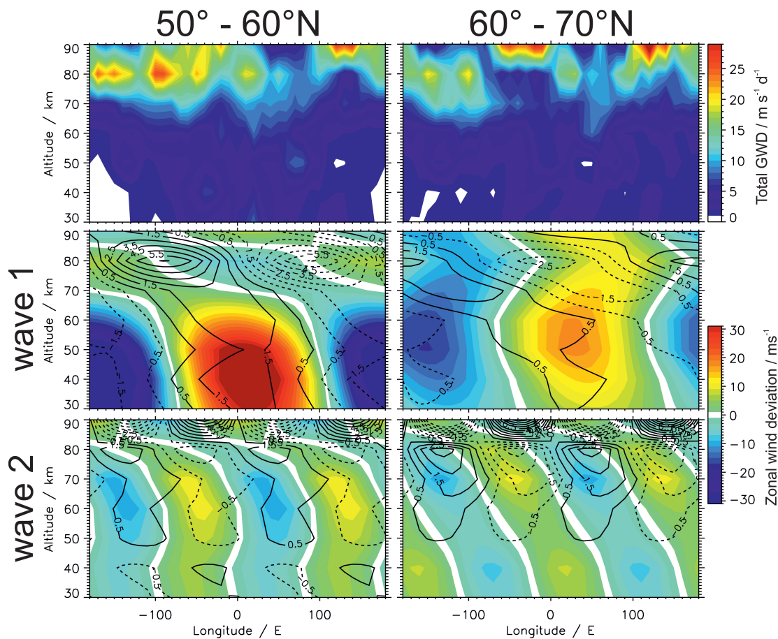
Fig. 3. Absolute GW drag in Period II filtered for different wavenumbers. Data are derived from SABER data.
