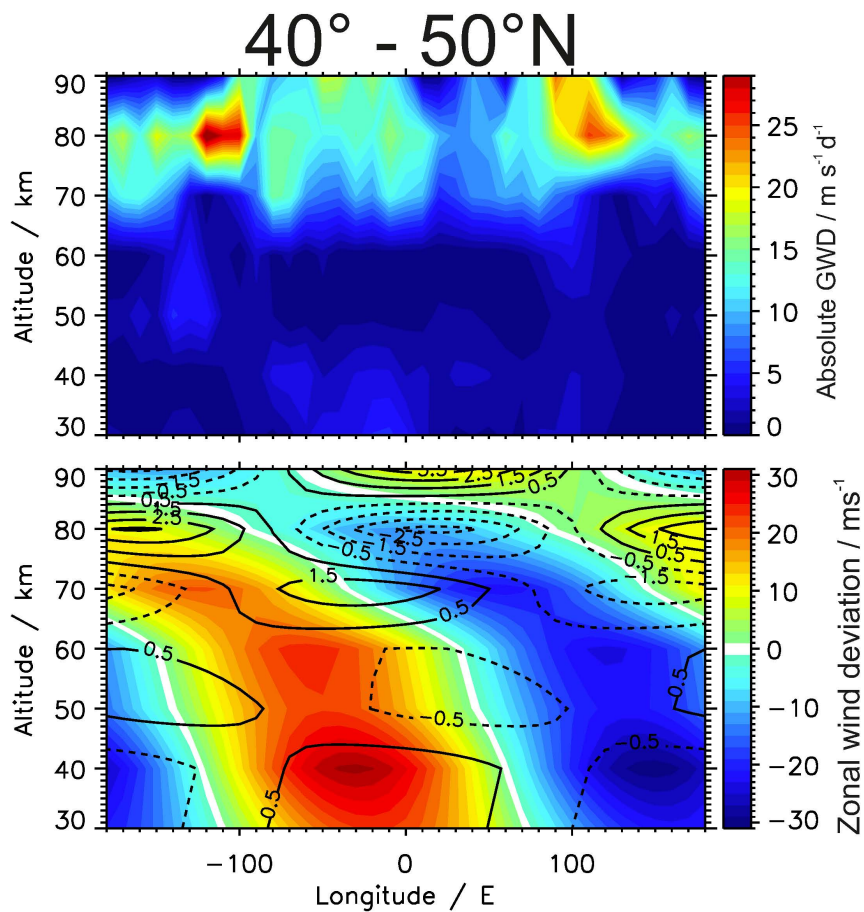
Fig. 2. Abolute GW drag averaged between 40 and 50°N in Period I. Data are derived from SABER data.
