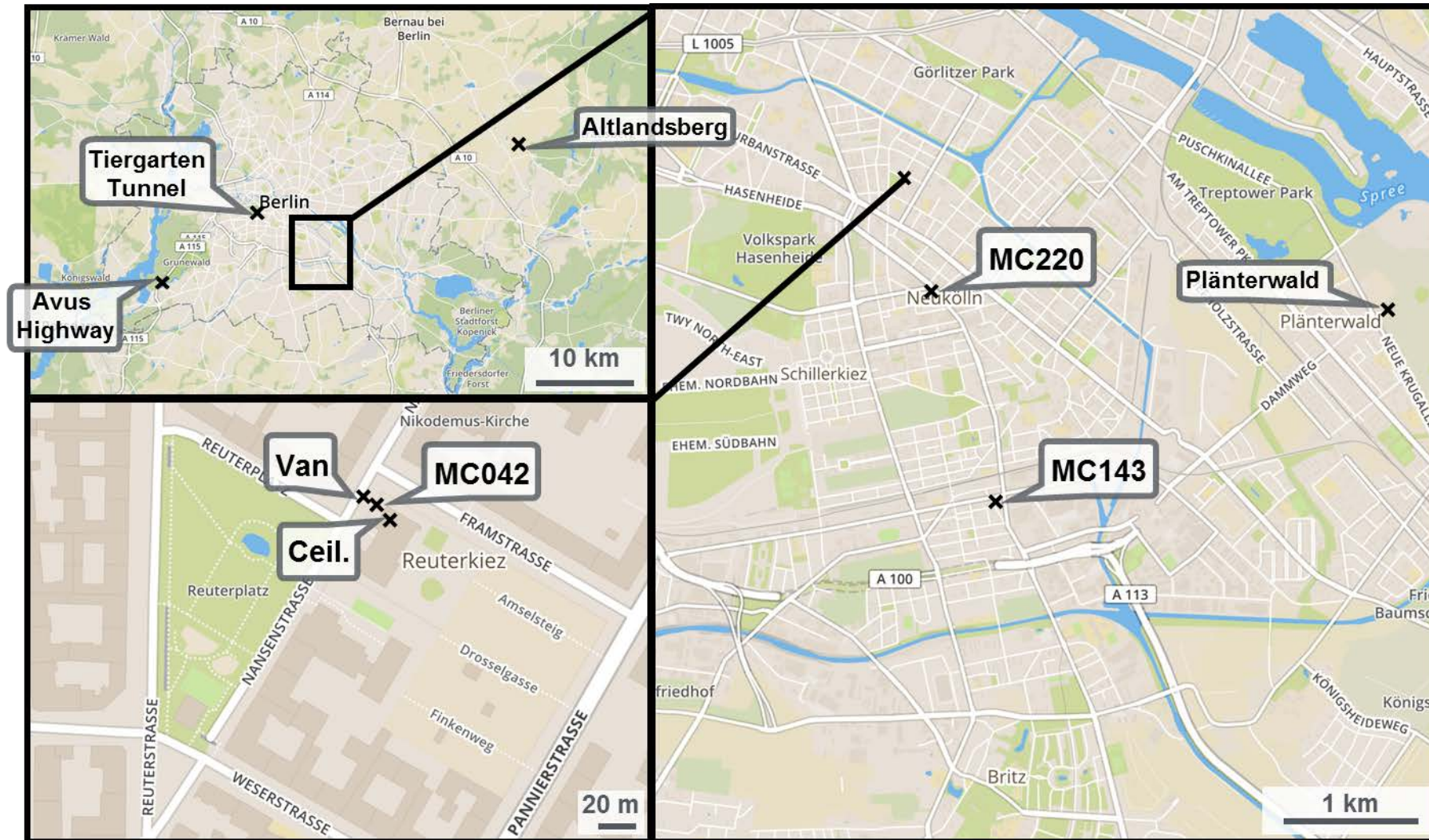
Figure 1. Location of the measurement station (MC042) and measurement van in Neukölln, Berlin. Maps show increasingly larger scale. The ‘x’ indicate sampling locations, with MC220 and MC143 indicating stations that record traffic counts. Map images from OpenStreetMap.
