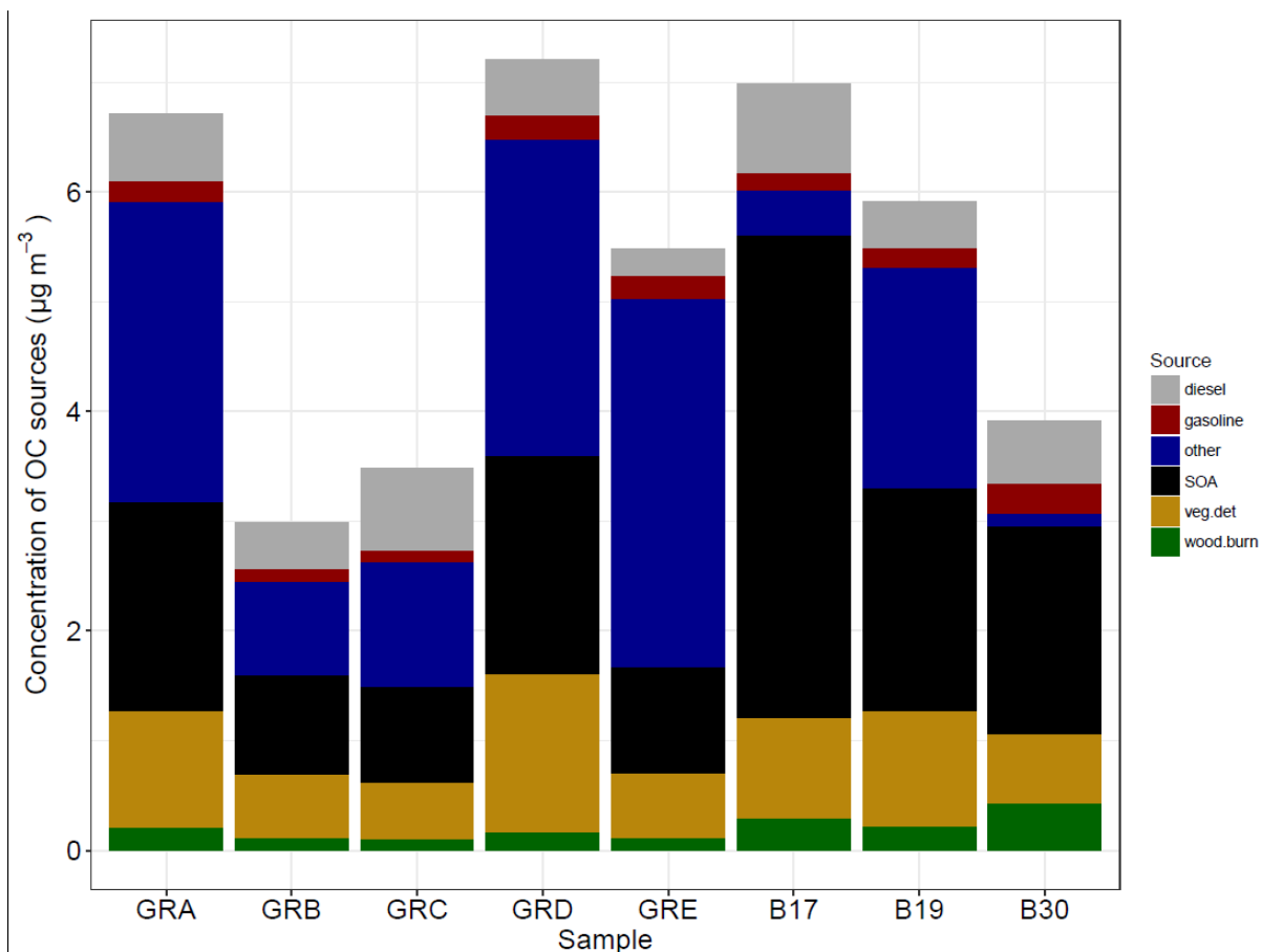
Figure 10. Source contributions attributed to the OC fraction of the PM 10 filter samples by filter groups, where GRA=Group A, GRB=Group B, etc. and B17, B19, B30 are individual filters. More information on the filter groups, including a some basic composition information and backtrajectory origin can be found in Table 3.
