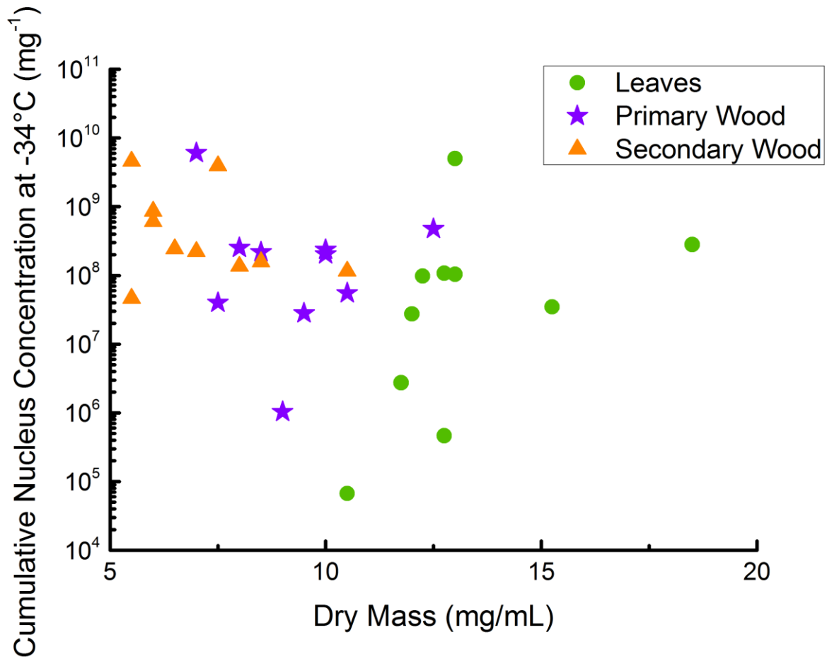
Figure 5: Scatterplot of dry mass (dry residues of the different filtered extracts) and cumulative nucleus concentration at -34 °C per sample mass. The dry mass is the mass we were able to extract with the 50 mg/mL suspensions. The data show that secondary wood, which contained mostly the highest INM concentrations and lowest variations between different samples, also contained the lowest extractable mass. Therefore INM ratios in the extractable content of the different samples were highest in secondary wood samples.
