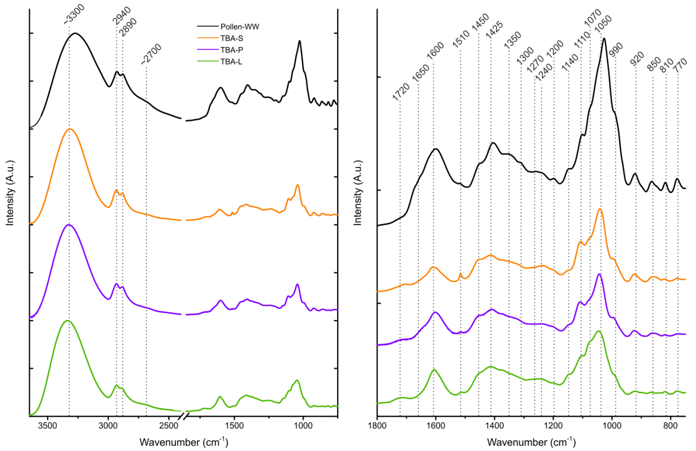
Figure 7: FTIR spectra of the TBA extracts (leaves in green, primary wood in violet and secondary wood in orange) and birch pollen washing water (black). Left: the whole spectrum between 3650 \text{cm}^{-1} and 750 \text{cm}^{-1} . Right: enlarged right side of the spectrum between 1800 \text{cm}^{-1} and 750 \text{cm}^{-1} . Possible band assignments are given in Table 3.
