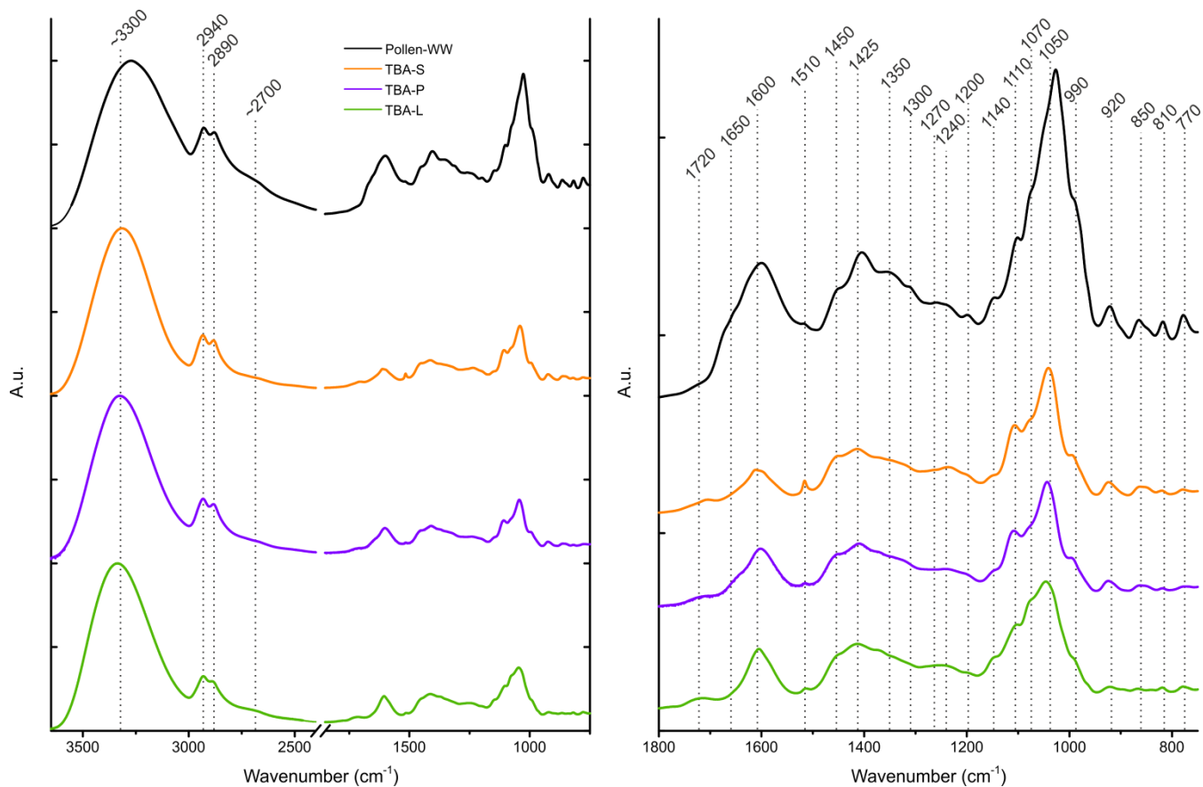
Figure 6: FTIR spectra of the TBA extracts (leaves in green, primary wood in violet and secondary wood in orange) and birch pollen washing water (black). Left: the whole spectrum between 3650\text{ cm}^{-1} and 750\text{ cm}^{-1} . Right: enlarged right side of the spectrum between 1800\text{ cm}^{-1} and 750\text{ cm}^{-1} . Possible band assignments are given in Table 2.
