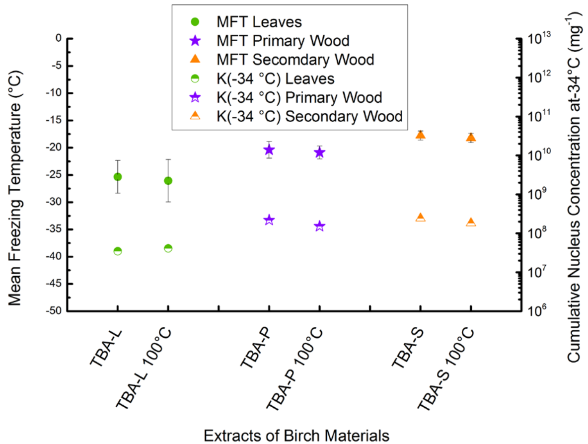
5 Figure 5: Results of the heat treatment of the different TBA extracts. Leaves are marked with green circles, primary wood with violet stars and secondary wood with orange triangles. The left value belongs to the untreated sample, the right value to the sample treated with 100 °C for an hour. Filled symbols represent the mean freezing temperature and correlate with the left Y-axis, half filled symbols represent the cumulative nucleus concentration as -34 °C per mg extracted sample and correlate with the right Y-axis.
