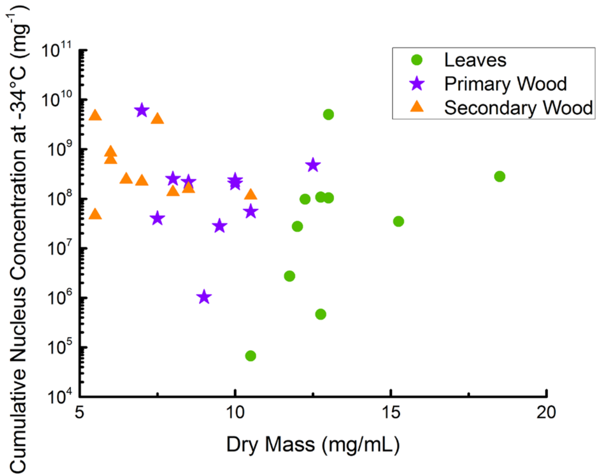
5 Figure 4: Scatterplot of dry mass (dry residues of the different filtered extracts) and cumulative nucleus concentration at -34°C per sample mass. The dry mass is the mass we were able to extract with the 50 mg/mL suspensions. The data show that secondary wood, which contained mostly the highest INM concentrations and lowest variations between different samples, also contained the lowest extractable mass. Therefore INM ratios in the extractable content of the different samples were highest in secondary wood samples.
