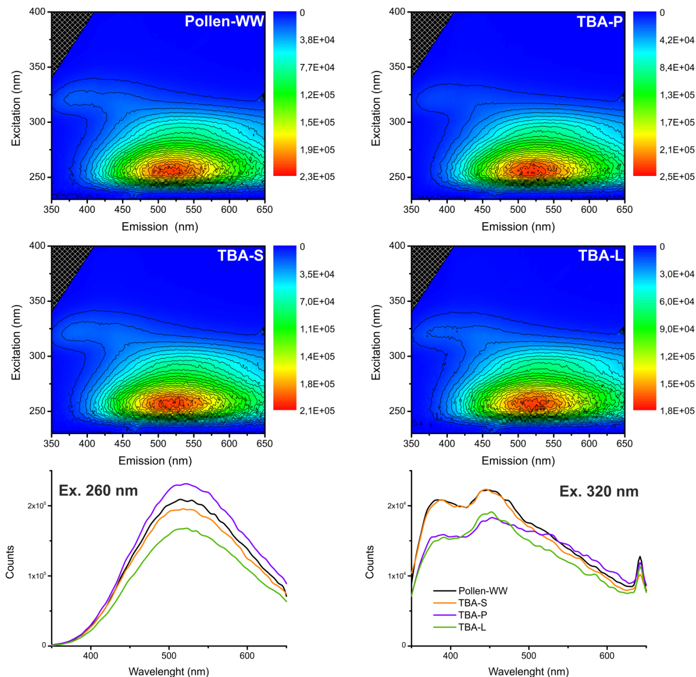
5 Figure 7: Top: fluorescence maps of pollen washing water (top left), and the extracts of TBA – secondary wood (bottom left), primary wood (top right) and leaves (bottom right). The excitation wavelength is shown on the y-axis, the emission wavelength on the x-axis and the corresponding counts are portrayed in colour (see colour bars right). Intensity correlates with brightness, level lines are included for the better visibility of the weaker double band on the right side of the map. Bottom: Emission-spectra of all four samples at the wavelengths 260 nm (left) and 320 nm (right). The band at 640 nm in the 320 nm emission-spectrum is an artefact due to second order excitation.
