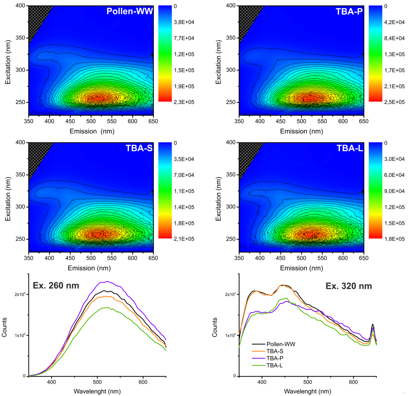
Figure 7: Top: fluorescence maps of pollen washing water (top left), and the extracts of TBA—secondary wood (bottom left), primary wood (top right) and leaves (bottom right). The excitation wavelength is shown on the y axis, the emission wavelength on the x axis and the corresponding counts are portrayed in colour (see colour bars right). Intensity correlates with brightness, level lines are included for the better visibility of the weaker double band on the right side of the map. Bottom: Emission spectra of all four samples at the wavelengths 260 nm (left) and 320 nm (right). The band at 640 nm in the 320 nm emission spectrum is an artefact due to second order excitation.
