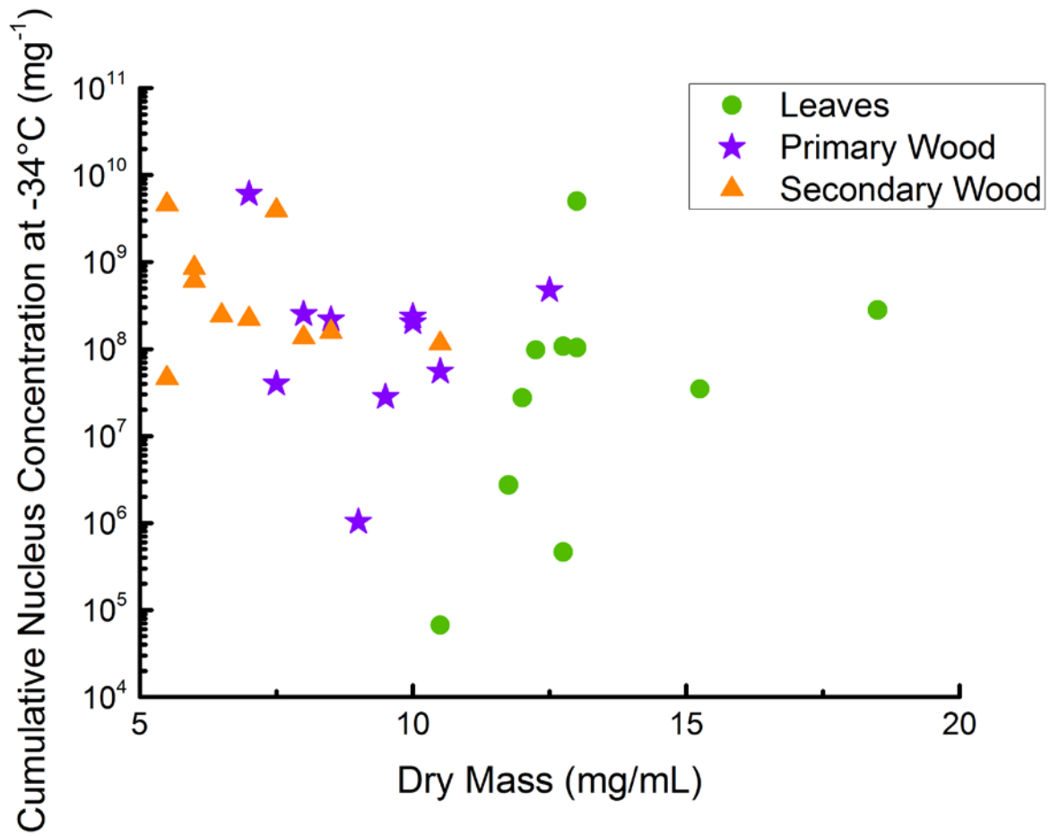
5 | Figure 5: Scatterplot of dry mass (dry residues of the different filtered extracts) and cumulative nucleus concentration at -34 °C per sample mass. The dry mass is the mass we were able to extract with the 50 mg/mL suspensions. The data show that secondary wood, which contained mostly the highest INM concentrations and lowest variations between different samples, also contained the lowest extractable mass. Therefore INM ratios in the extractable content of the different samples were highest in secondary wood samples.
