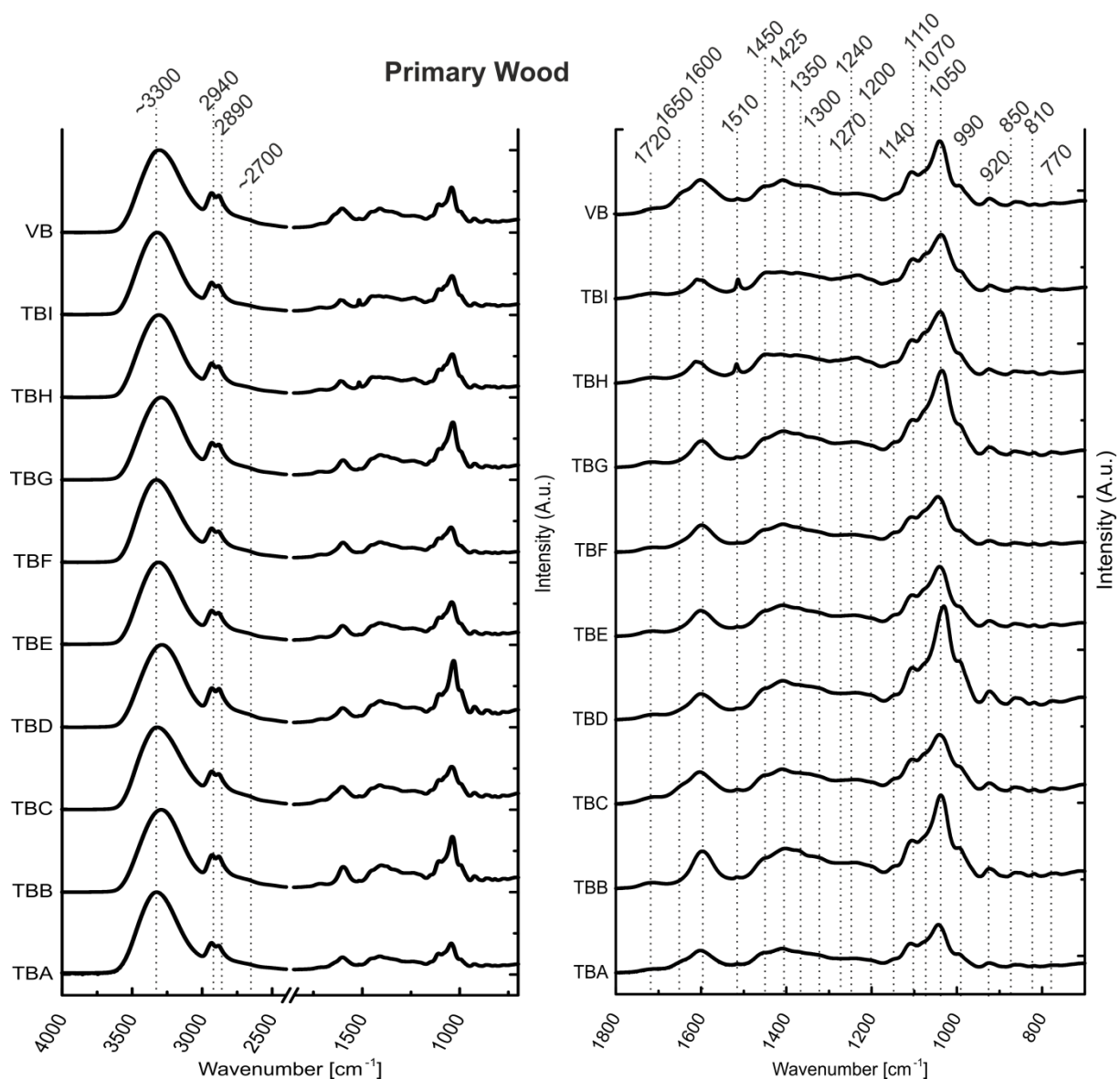
Figure S2: The IR spectra of the all analysed extracts of primary woods. Left: the whole spectral range, right: a close-up on the spectra below 1800 \text{cm}^{-1} .
