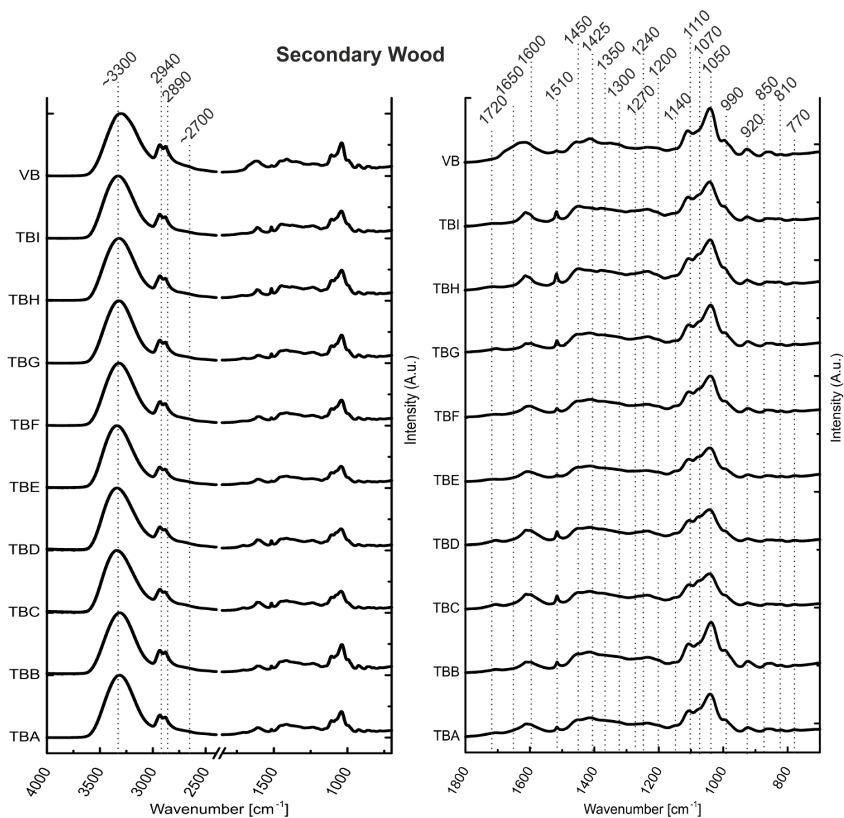
Figure S3: The IR spectra of the all analysed extracts of secondary woods. Left: the whole spectral range, right: a close-up on the spectra below 1800 \text{cm}^{-1} .
