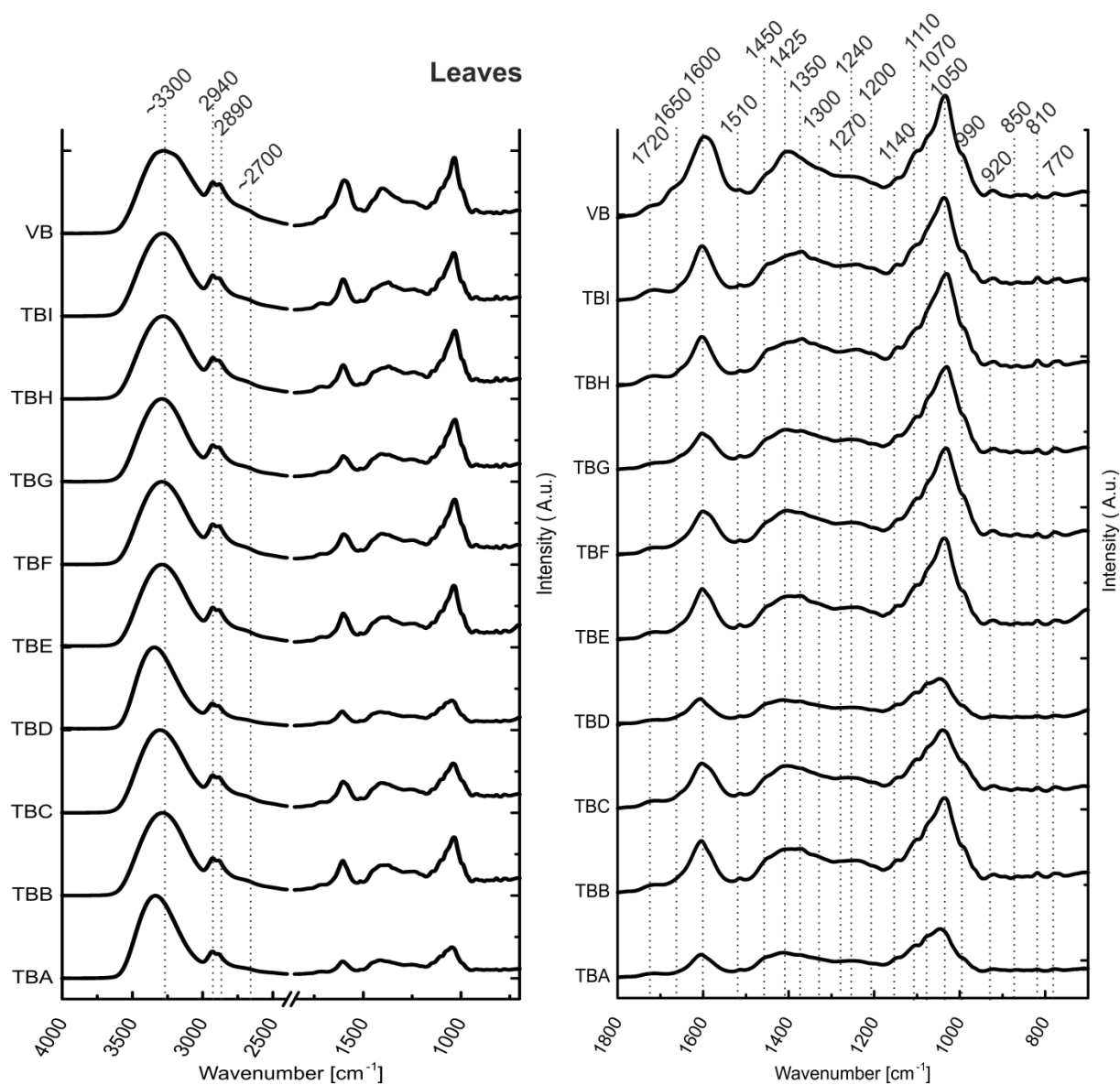
Figure S1: The IR spectra of the all analysed extracts of leaves. Left: the whole spectral range, right: a close-up on the spectra below 1800 cm -1 .
