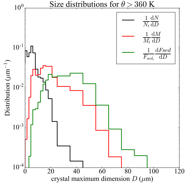
Figure 8. Average ice crystal size distribution within cirrus clouds during ATTREX 2014 flights, above \theta = 360 \text{ K} . In black, number distribution; in red, mass distribution; in green, mass flux distribution. The distributions shown are composites of 2DS and FCDP measurements. The size considered is the maximum dimension, the diameter for spherical particles. It should be mentioned that the size retrieved by the FCDP is not strictly exact because the retrieval of size distribution from scattered light assumes spherical particles. The sedimentation speed needed for the mass flux computation are computed using the formula of Heymsfield and Westbrook (2010).
