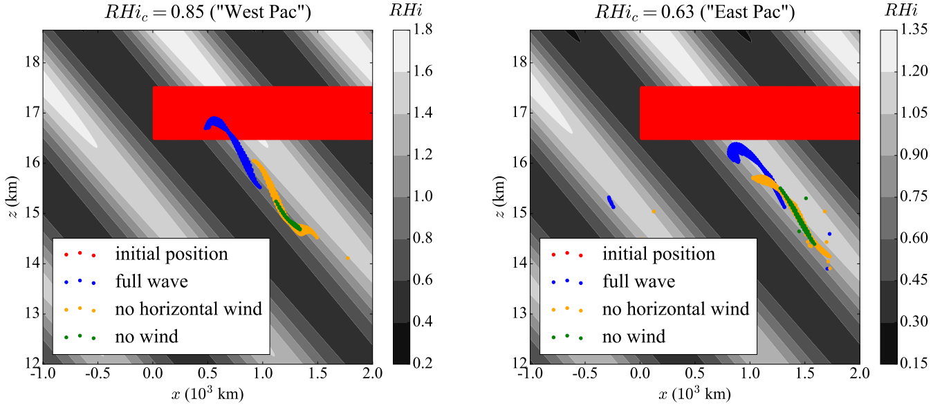
Figure C1. Same as Fig. 6, but including ice crystal positions from simulations with the wave vertical wind accounted for but not the horizontal one (orange). As in Fig. 6, the blue dots are the ice crystals' positions for the full simulation (wave advection and temperature fluctuations), and the for the green dots both the horizontal and vertical winds induced by the wave have been neglected. The initial ice crystal radius used in both cases for all crystals is 5 \mu\text{m} .
