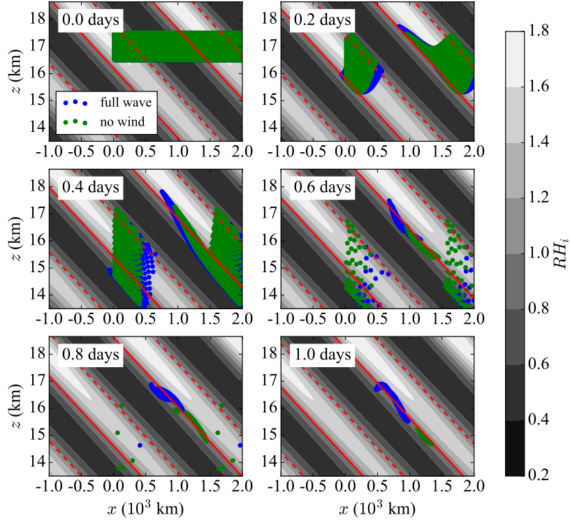
Figure 5. Simulations of ice crystal growth and sedimentation in an idealized wave field at RH_{i_c} = 85\% . Different integration times are displayed, up to half a wave period, i.e. one day. The black and white background represents the RH_i spatial variability and the colored dots correspond to the position of the ice crystals. The different colors correspond to simulations with different processes (un)accounted for: the blue dots represent the ice crystals’ positions for the full simulation (wave advection and temperature fluctuations) whereas for the green dots both the horizontal and vertical winds induced by the wave have been neglected. The solid and dashed red lines respectively correspond to the locations of the elliptic and saddle points; for both of those RH_i = 100\% . The initial ice crystal radius used for all crystals is 5 \mu\text{m} .
