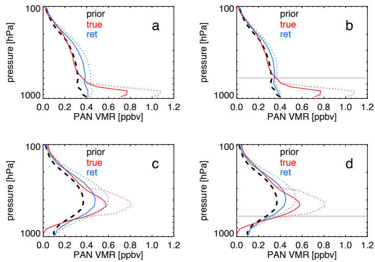
700 Figure 1: Simulated TES PAN retrievals for four different hypothetical conditions where the black dashed line shows the prior, the two red lines show two different true profiles, and the two blue lines show the retrieved profiles. The true profile exhibits a maximum in the vmr close to the surface in the upper panels (a and b), while the true profile peaks in the mid-troposphere in the lower panels (c and d). Panels on the left (a and c) show clear-sky retrievals while panels on the right (b and d) show retrievals where a cloud 705 with effective optical depth of 0.7 is placed at 600 hPa (dotted line). Corresponding averaging kernels are provided in the Supplementary Information.
