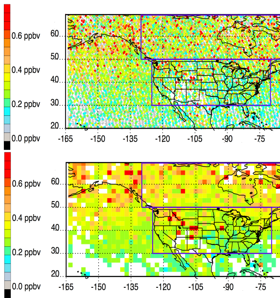
710 Figure 2: Average tropospheric PAN in retrievals (DOF > 0.6) during July 2006 – July 2009 (top), and those retrievals averaged in a 2°x2° grid (bottom). The white areas designate locations with less than 5 measurements during this period. The blue lines surround the regions included in the calculations in Figures 4 and 5: 125° W - 70° W, 30° N – 50° N and 130° W - 65° W, 50° N – 70° N.
