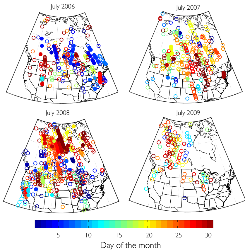
775 Figure 6: Successful TES PAN retrievals overlapping NOAA HMS smoke polygons for July 2006 to July 2009 colored by the day of the month. Filled circles denote the set of retrievals that also coincide with 510 hPa CO greater than 150 ppbv. This set of point is used to calculated PAN enhancement ratios relative to CO in Figure 8.
