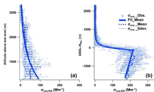
Fig. 6. Mean vertical distributions of \sigma_{\text{sca}} at 550 nm (in \text{Mm}^{-1} ) during the flight campaign for those cases of (a) clean PBL and (b) pollution in the lower layer of the PBL where PBL heights have been normalized to the same altitude. Blue dashed lines and light blue dots represent mean \sigma_{\text{sca}} vertical profiles and 1 s Nephelometer-measured \sigma_{\text{sca}} , respectively. Thick blue lines show the calculated fitting curves of the \sigma_{\text{sca}} profiles (see Eq. 6 and 7) and horizontal error bars represent the standard deviations at every 100 m level.
