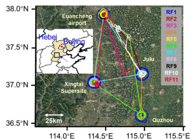
Fig. 1. Flight tracks of the 11 research flights conducted over Hebei Province in the North China Plain during the May–June 2016.
