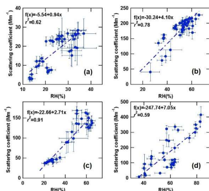
Fig. 9. \sigma_{\text{sca}} at 500 nm as a function of relative humidity (RH, in %) for those cases when the PBL was (a) clean and dry, (b) polluted in the lower PBL, (c) polluted in the upper PBL, and (d) polluted in multiple layers of the PBL. The linear regression best-fit lines through the data are shown (dashed lines). The regression relationships and coefficients of determination are given in each panel.
