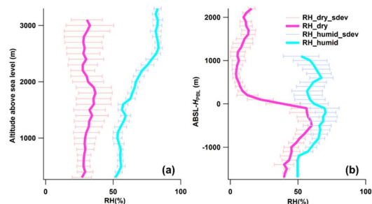
Fig. 7. Mean vertical profiles of relative humidity (%) during the flight campaign for those cases of (a) clean PBL and (b) pollution in the lower layer of the PBL where PBL heights have been normalized to the same level. Magenta lines represent data collected under dry
