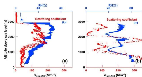
Fig. 8. Vertical distributions of \sigma_{\text{sca}} at 550 nm (red) and relative humidity (RH, blue) for the enrichment of aerosols in the upper layer of the PBL on 2 June (a) and in multiple layers of the PBL on 6 June (b).
