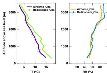
Fig. 2. Vertical profiles of temperature (T, left) and relative humidity (RH, right) from radiosonde and airborne measurements made on 8 May 2016 over Xingtai supersite. Horizontal bars represented standard deviations.
