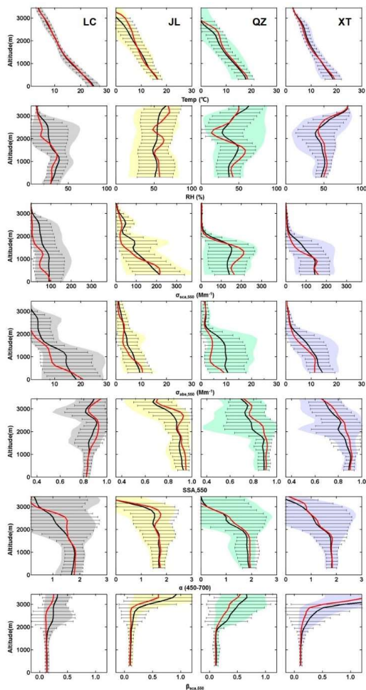
Fig. 4. Mean vertical distributions of (from the top row to the bottom row) temperature ( ^{\circ}\text{C} ), relative humidity (%), \sigma_{\text{sca}} at 550 nm ( \text{Mm}^{-1} ), \sigma_{\text{obs}} at 550 nm ( \text{Mm}^{-1} ), SSA at 550 nm, Ångström exponent ( \alpha ), and \beta_{\text{sca}} at 550nm over LC, JL, QZ and XT (from left column to right column, respectively). Black and red lines represent the mean and the median, respectively, and horizontal bars are standard deviations at every 150-m level. The colored shaded areas represent the 10 th and 90 th percentiles of the data.
