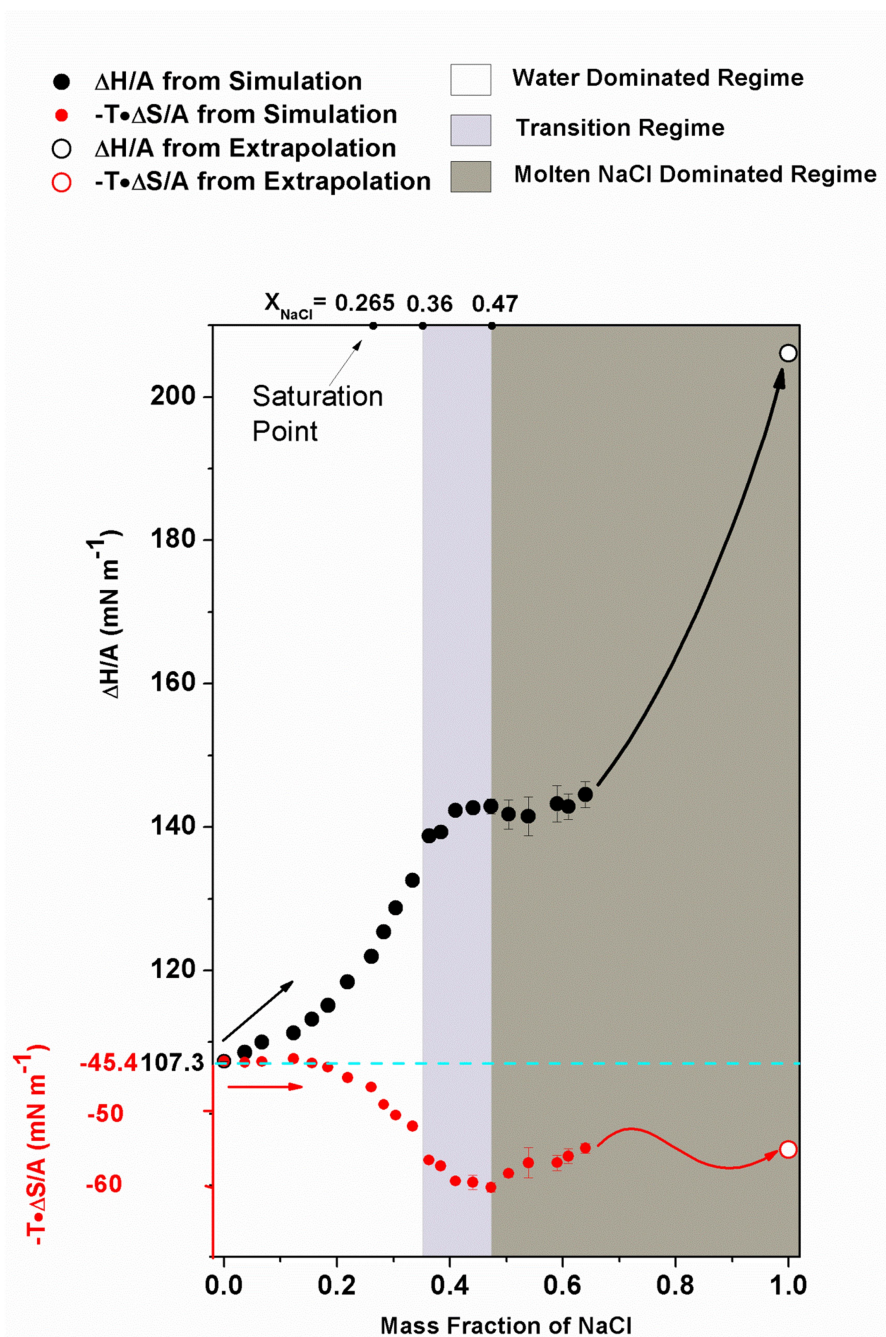
Figure 6. The excessive surface enthalpy and entropy per unit area ( \frac{\Delta H}{A} and \frac{T\Delta S}{A} ) of different NaCl solution concentrations. \frac{\Delta H}{A} (black circles) and -\frac{T\Delta S}{A} (red circles) are shown as a function of mass fraction of NaCl. The solid circles are obtained from simulation directly, and the open circles are obtained from the extrapolation of corresponding properties of molten NaCl. The cyan dashed line is only an auxiliary line for clearer view. Shaded areas are the same as in Figure 4.
