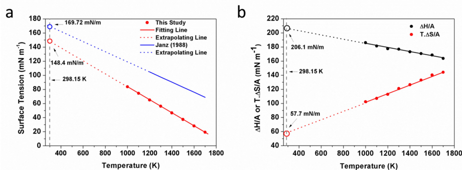
5 Figure 5. The surface tension, enthalpic part ( \frac{\Delta H}{A} ) and entropic part ( \frac{T \cdot \Delta S}{A} ) of molten NaCl at different temperature. (a) The equation in Janz's study (1988) is \sigma_{NaCl} = -0.07188 \cdot T + 191 (blue solid line). The fitting line based on our data (red solid line) is \sigma_{NaCl} = -0.0922 \cdot T + 175.91 . The red and blue open circles represent the extrapolated value of surface tension in simulation and reality. (b) The black and red open circles represent the extrapolated \frac{\Delta H}{A} and \frac{T \cdot \Delta S}{A} of molten NaCl at 298.15 K, respectively.
