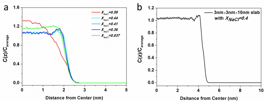
5 Figure 7. The ratio of Na + concentration at different positions ( C_z ) to the average concentration of the whole system ( C_{average} ). (a) The solution with x_{NaCl} = 0.59 (red line) is on behalf of the solution in the molten NaCl-dominated regime (red line), the solution x_{NaCl} = 0.44, 0.41 and 0.36 (blue lines) represent the solution in transition regime, and the solution x_{NaCl} = 0.037 (green line) represents the solution in the water-dominated regime. (b) The density profile obtained from a 3\text{ nm} \times 3\text{ nm} \times 10\text{ nm} solution slab in which NaCl mass fraction is about 0.4.
