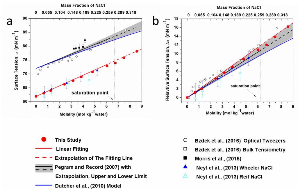
Figure 3. Surface tension (a) and relative surface tension (b) defined as \Delta\sigma = \sigma_{\text{solution}} - \sigma_{\text{water}} as a function of the concentration of NaCl. The \sigma_{\text{water}} in the Morris et al. (2015) study was not determined, thus the corresponding \Delta\sigma is not shown in panel b.
