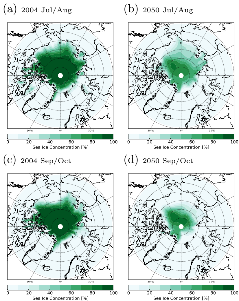
Figure 2. SIC in 2004 and 2050 for late summer (Jul/Aug) and for early autumn (Sep/Oct).
