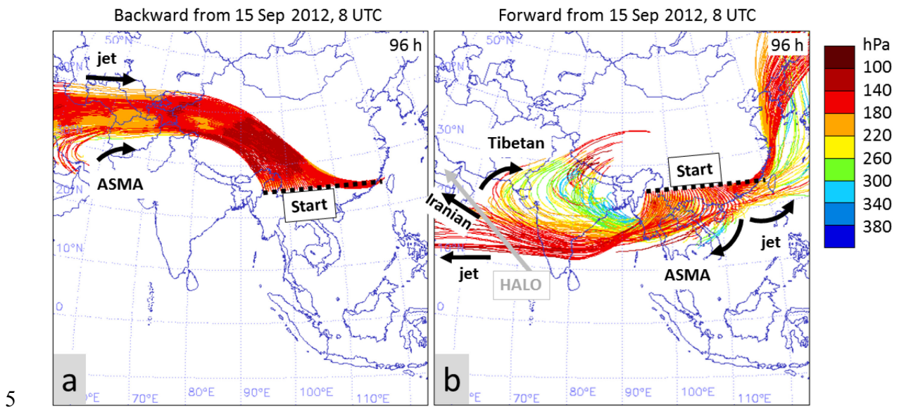
10 Figure A2: Four day backward (panel a) and four day forward (panel b) trajectories, starting between 12 and 14 km altitude. The trajectories start from a plane intersecting the eastern ASMA edge when the air mass measured by HALO during POI3 was there. The wind field is strongly divergent at the eastern ASMA flank, where the subtropical jet separates from the anticyclone. During the time covered by the trajectories the anticyclone split into a Tibetan and an Iranian part, just where HALO was passing through.
