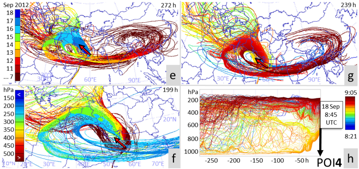
5 Figure A3: As Fig. 3, but for POI4. This flight segment covers the dive from the UT into the middle troposphere. The interval for POI4 is chosen such that anticyclonic motion is much slower compared to the ASMA circulation above: Air from the highest altitudes of POI4 does not nearly circle the ASMA within 300 h, while air from POI3/5 needs about 200 h and 280 h, respectively (Figs. 3, A4). The source regions contributing to POI4 primarily depend on the actual flight altitude, i.e. the sequence of air masses encountered during descent is mirrored during the following ascend.
