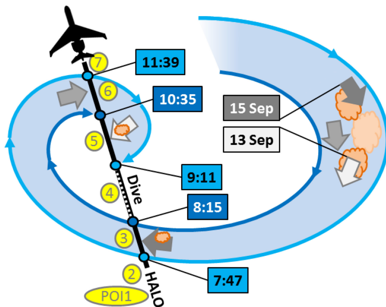
5 10 Figure 5: Schematic of the filament of UT ASMA air that was transected by HALO during the ESMVal campaign. The encountered air parcels all had a similar genesis: UT air travelling in the ASMA fringe was to different degrees entrained by deep convection at the eastern ASMA flank, then continuing along the southern flank of the anticyclone to the respective measurement locations. POI3 provides the most direct view of the eastern ASMA flank. The schematic is in ASMA centered coordinates, with relative positions of air masses (grey arrows) and convection (orange clouds) indicated. The interior trajectory of the filament and corresponding times of measurement are indicated by dark blue and the exterior trajectory is light blue. Grey shades and white indicate the air masses encountered during the respective three periods of interest (POI3/5/6), and to the corresponding date they passed the eastern flank.
