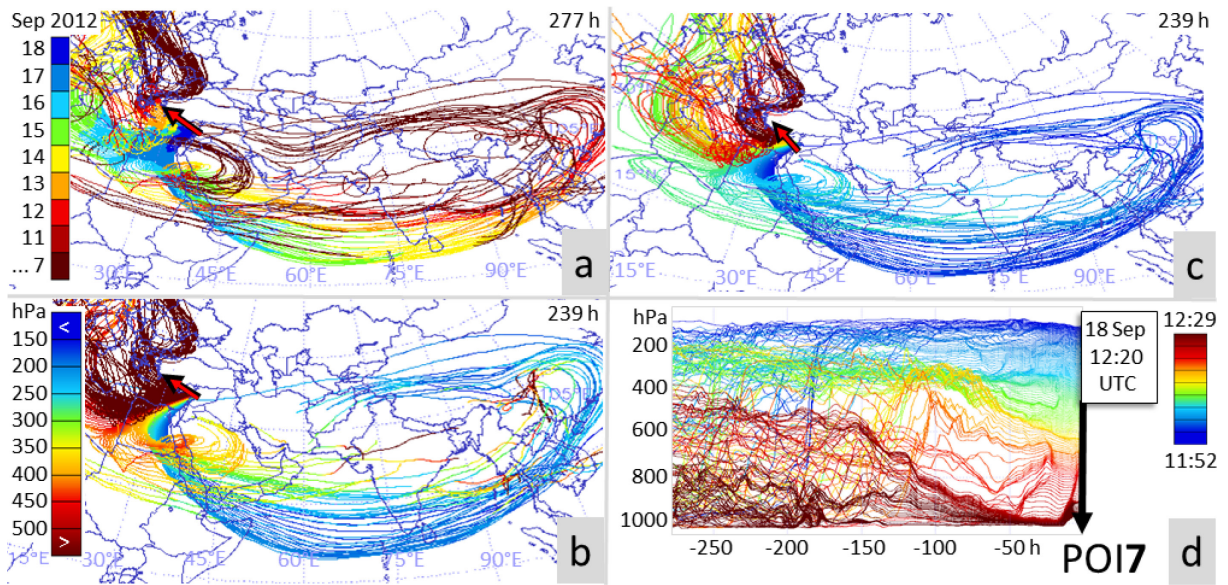
Figure A6: As Fig. 3, but for POI17. This flight segment covers the descent into Larnaca.
