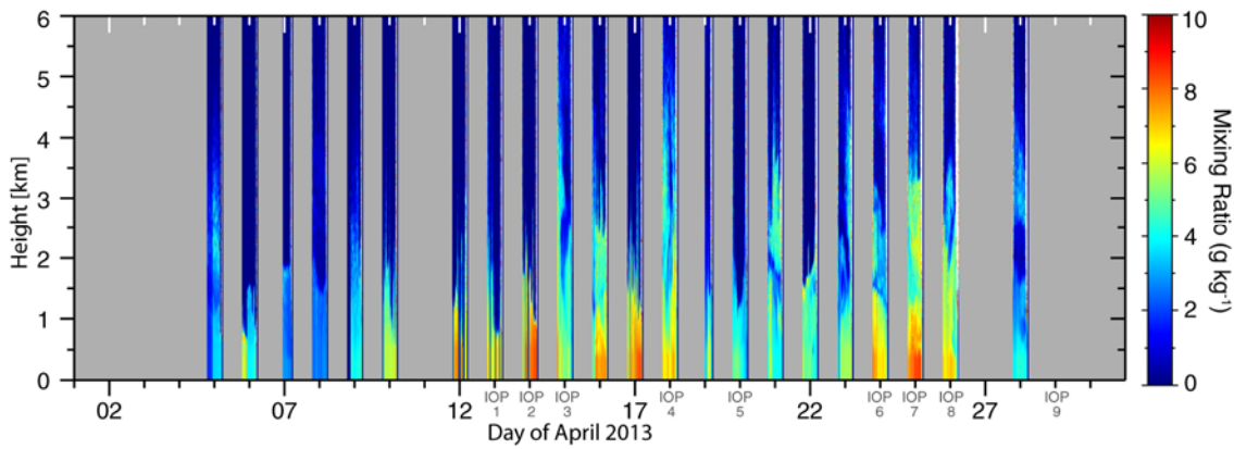
Figure 9: Calibrated nighttime observations at KRA of the water vapour mixing ratio for April 2013 during HOPE-Jülich obtained from Polly XT data—that were calibrated automatically with the integrated water vapour provided by a co-located microwave radiometer. Adapted from Foth et al. (2015).
