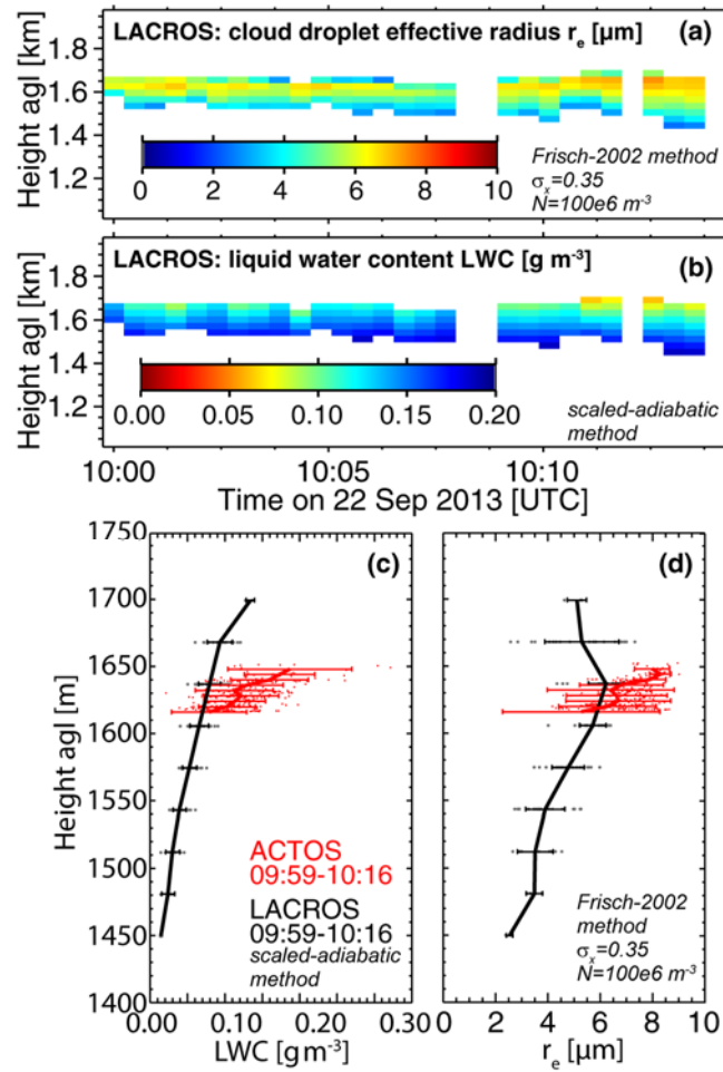
Figure 12: Stratocumulus observation at the Melpitz site on 22 September 2013. Time-height cross sections of Vertical profiles of (a) cloud droplet effective radius and (b) liquid water content as observed from ground-based remote sensing with LACROS, and (c-d): cloud droplet Profiles of single data points, mean, and standard deviation (horizontal bars) of (c) liquid water content and (d) effective radius as observed in-situ with ACTOS (red) and retrieved from LACROS (black) for the time period shown in (a) and (b). Scaled-adiabatic method is based on Merk et al. (2016), Frisch-2002 method is based on Eq. 5 of Frisch et al. (2002).
