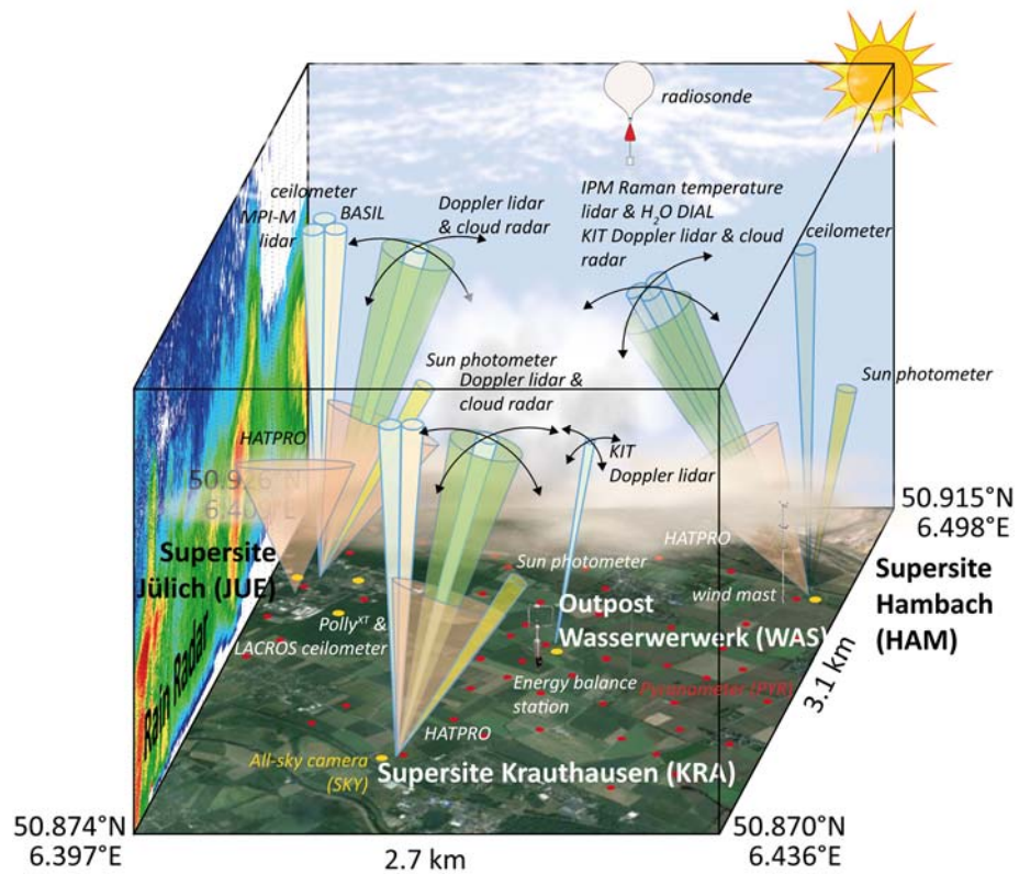
Figure 1: Setup of the HOPE-Jülich campaign showing the (a) Location of the three supersites Jülich (JUE), Hambach (HAM), and Krauthausen (KRA) as well as the outpost Wasserwerk (WAS) with their main instrumentation. The cones during HOPE-Jülich and arrows illustrate the field-of-view and scanning capabilities of the specific remote-sensing instruments. (b) Location of the instrumentation during HOPE-Melpitz.
