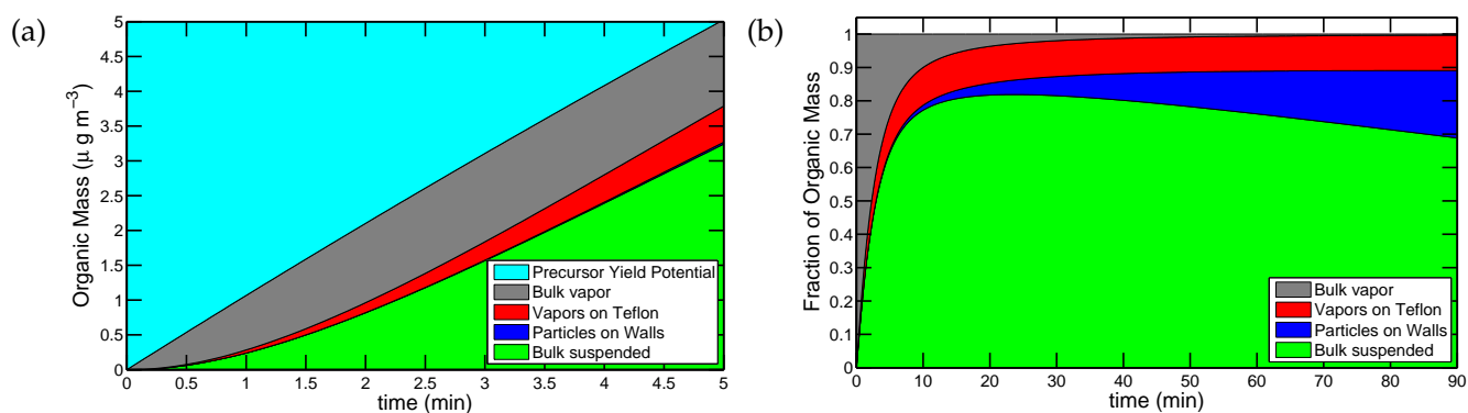
Figure 6. Mass distribution among organic reservoirs. The first five minutes of Experiment 1 (a) show the different reservoirs of organic mass including a substantial fraction of uncondensed vapors (gray). The buildup of the bulk vapors demonstrates that there is a significant delay between the formation of low volatility compounds and the condensation of these compounds onto particles. This results in lower detected yields during chamber experiments and the loss of vapors to the walls. The fraction of organics in each of the reservoirs over the first 90 minutes (b). At the beginning, all of the organics are in the bulk vapor reservoir. The bulk vapor fraction decreases as vapors condense or are lost to the walls and claim a larger fraction of total organic mass.
