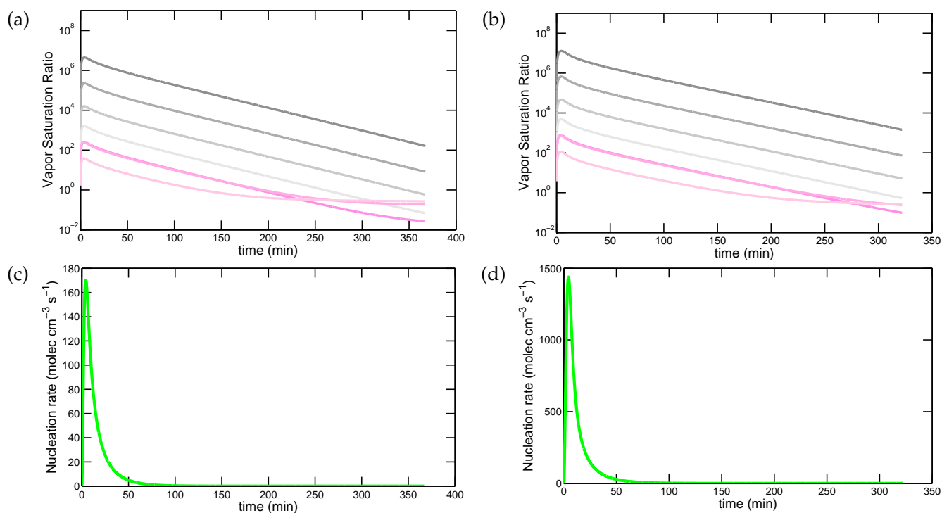
Figure 7. Vapor saturation ratios for smog-chamber experiments experiments. Simulated vapor saturation ratios in the CMU smog chamber for Experiment 1 (a) and Experiment 2 (b). The color of the line indicates the volatility bin, with the ELVOCs in shades of grey and LVOCs in shades of pink, and darker shades indicate lower volatility within the category. The saturation ratio of the least volatile ELVOC ( C^* = 10^{-8} \mu\text{g m}^{-3} , dark gray) can be used to predict nucleation rates based on CLOUD data, which are shown in the lower panels for Experiment 1 (c) and Experiment 2 (d). However, no nucleation was observed during these experiments.
