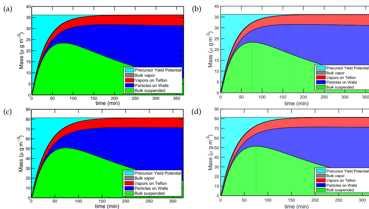
Figure 3. Dynamical simulation of \alpha -pinene SOA for two experimental conditions, using a monodisperse and polydisperse model. The simulations describe five different reservoirs: unreacted precursor, vapors, suspended particles, deposited particles, and sorption to teflon, as shown in the legend. Experiment 1 monodisperse (a) and polydisperse (b) results. Experiment 2 monodisperse (c) and polydisperse (d) results. The monodisperse model uses a "condensation sink diameter" to approximate the rate that organics condense onto particles. This serves as a good proxy for a polydisperse model that accounts for the different condensation sinks for a polydisperse seed distribution.
