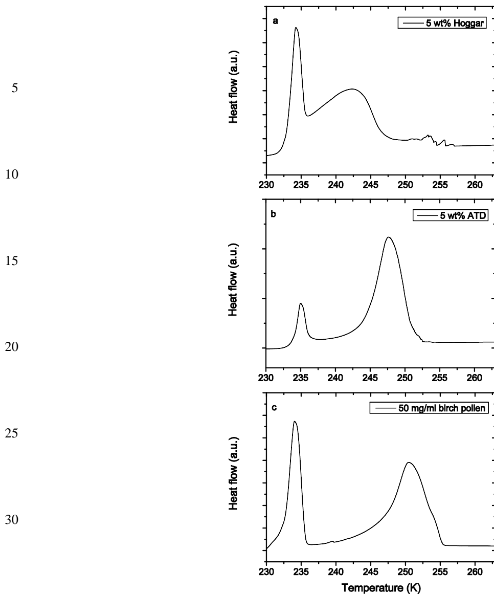
Figure 1. DSC thermograms of emulsion experiments for 1 K/min cooling rate. Panel a: Hoggar Mountain dust emulsion sample with homogeneous freezing peak at \sim 234 K and heterogeneous freezing peaking at \sim 244 K. The spikes around 253 K are due to latent heat release by a few very large water droplets containing Hoggar Mountain dust. Panel b: ATD emulsion sample. The broad peak at \sim 248 K stems from heterogeneous freezing induced by ATD particles present in many droplets, the narrow peak at \sim 235 K from homogeneous freezing of a few pure water droplets. Panel c: Birch pollen washing water emulsion sample with the heterogeneous freezing peak at \sim 250 K.
