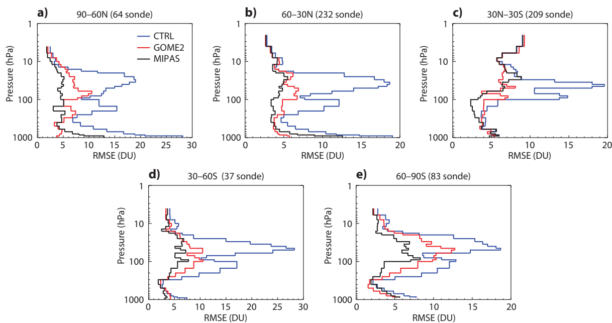
Figure 12. Fit of the ozone analyses from three experiments to ozone sondes given in terms of the RMSE over five latitudinal bands. The comparisons were computed by averaging over Aug - Oct 2008. The three analyses were taken from Exp/Ctrl (blue lines), and the two Exp/PERT experiments assimilating also the reprocessed GOME-2 NPO 3 (red lines) and MIPAS LPO 3 (black lines) from the Ozone-CCI. The latitudinal band each panel refers to and the number of ascents included in the average can be found in the corresponding panel title. Data are in Dobson Unit (DU).
