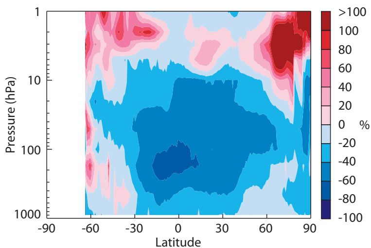
Figure 5. Vertical cross-section of the difference between the estimated and the provided uncertainty relative to the provided uncertainty for GOME-2 NPO 3 over the period Jul-Oct 2008. Negative (positive) values in blue (red) colours mean that the provided uncertainty is larger (smaller) than that estimated with the Desroziers et al. (2005) method. Data are in %.
