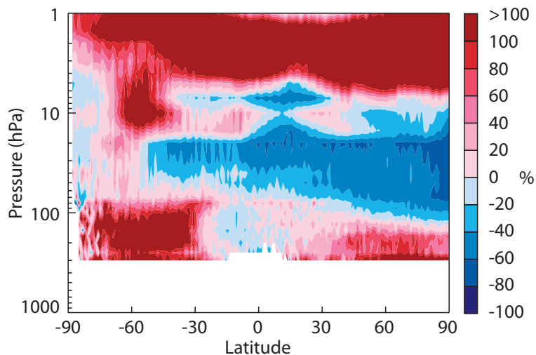
Figure 6. As in Figure 5 but for the CCI MIPAS LPO 3 data.
