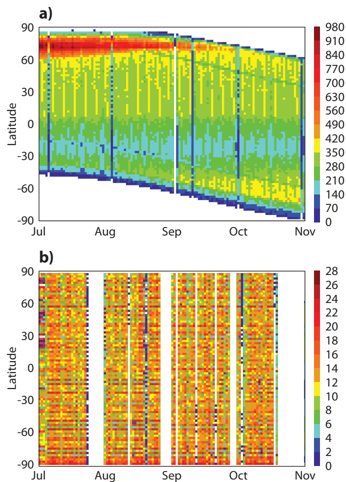
Figure 1. Data coverage and daily count binned in 2° latitudinal bands for the CCI GOME-2 (top panel) and the CCI MIPAS (bottom panel) data. The two colour scales are different. The colour scale used for GOME-2 (panel a) varies from 0 (dark blue) to 980 (dark red) observations with a step of 70; the one used for MIPAS ranges from 0 (dark blue) to 28 (dark red) observations with a step of 2.
