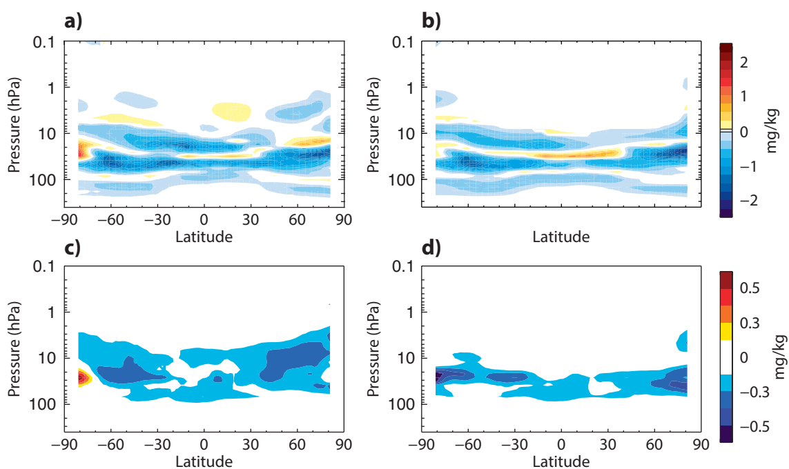
Figure 9. Top panels: Change in the zonal mean differences between the MLS retrievals and collocated ozone analyses from the perturbation experiment compared to the Exp/Ctrl for Aug-Oct 2008. The perturbation experiment is Exp/GOME2 in the left panel, and Exp/MIPAS in the right panel. Negative (positive) values in blue (red) colours indicate a decrease (an increase) in the mean in the Control and thus a degraded fit to MLS ozone profiles. Data are in mg/kg. The colour scale ranges from -2.5 mg/kg (dark blue colour) to +2.5 mg/kg (dark red colour) with a step of 0.25 mg/kg. Bottom panels: As a), but for the standard deviation of differences. The colour scale ranges from -0.6 mg/kg (dark blue colour) to +0.6 mg/kg (dark red colour) with a step of 0.1 mg/kg.
