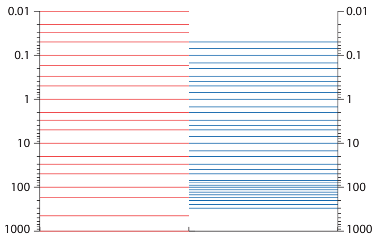
Figure 2. Schematic of the vertical coverage and vertical resolution provided by the CCI GOME-2 (red lines) and the CCI MIPAS (blue lines) retrieval algorithms. The vertical axis represents pressure in hPa. The surface pressure level for GOME-2 is for illustration purposes drawn at 1000 hPa.
