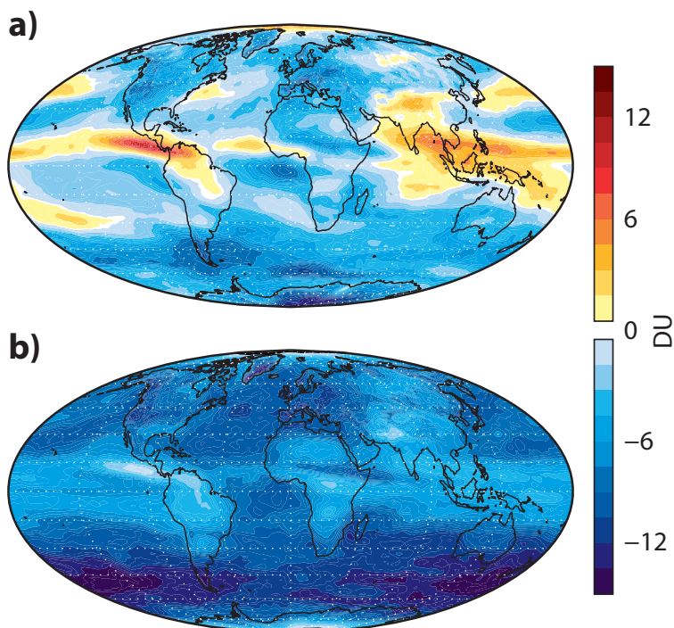
Figure 7. TCO 3 mean differences between the analyses from Exp/Ctrl and those from Exp/GOME2 (top) and Exp/MIPAS (bottom) computed for the period Aug-Oct 2008. Negative (positive) values in blue (red) colours mean that the additional instrument is increasing (decreasing) the TCO 3 amount compared to that obtained from the ozone datasets assimilated in Exp/Ctrl. Data are in DU. The colour scale ranges from -15 DU (dark blue) to +15 DU (dark red) with a step of 1.5 DU.
